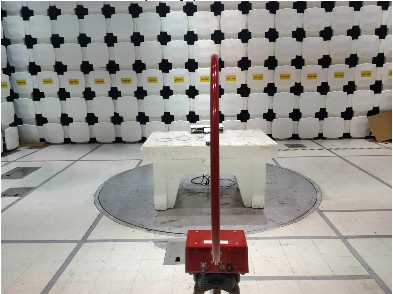
Setup Photograph Below 30 MHz
