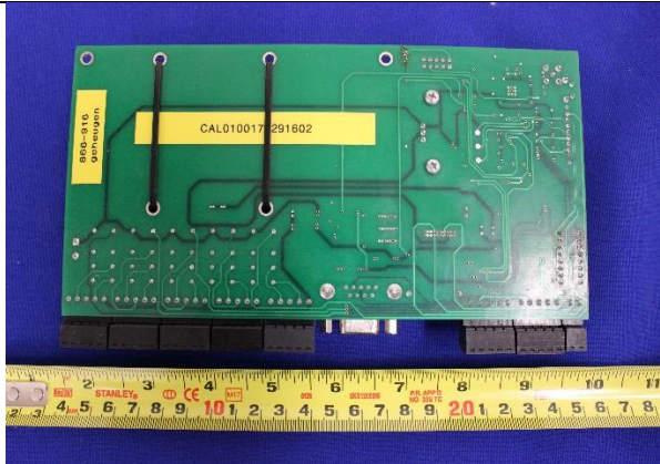
EUT – Telesto PCB Board Bottom View
