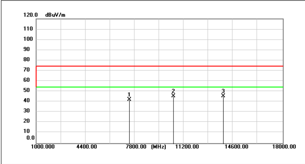
BLE_1M_TX_CH_19_Vertical
