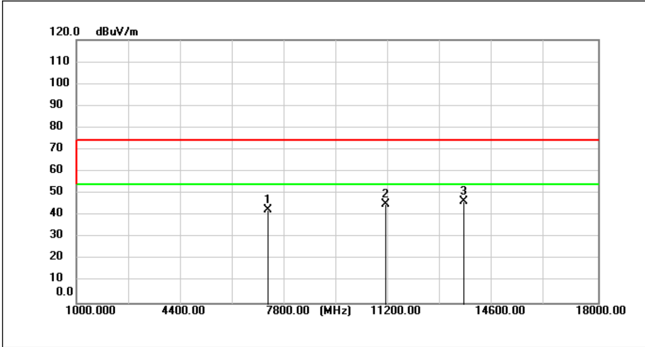
BLE_2M_TX_CH_19_Vertical
