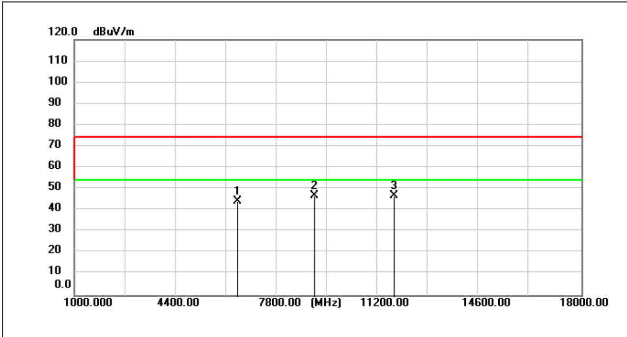
BLE_1M_TX_CH_00_Vertical
