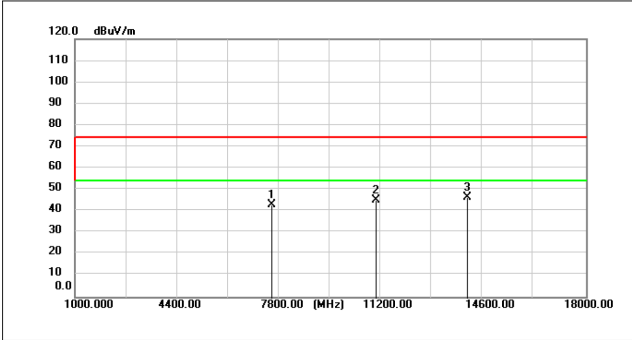
BLE_1M_TX_CH_39_Vertical
