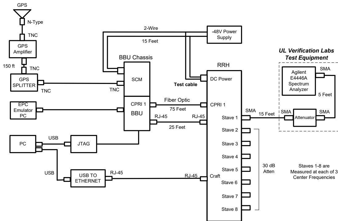
Conducted Emissions Tests Configuration - RRH to Spectrum Analyzer
