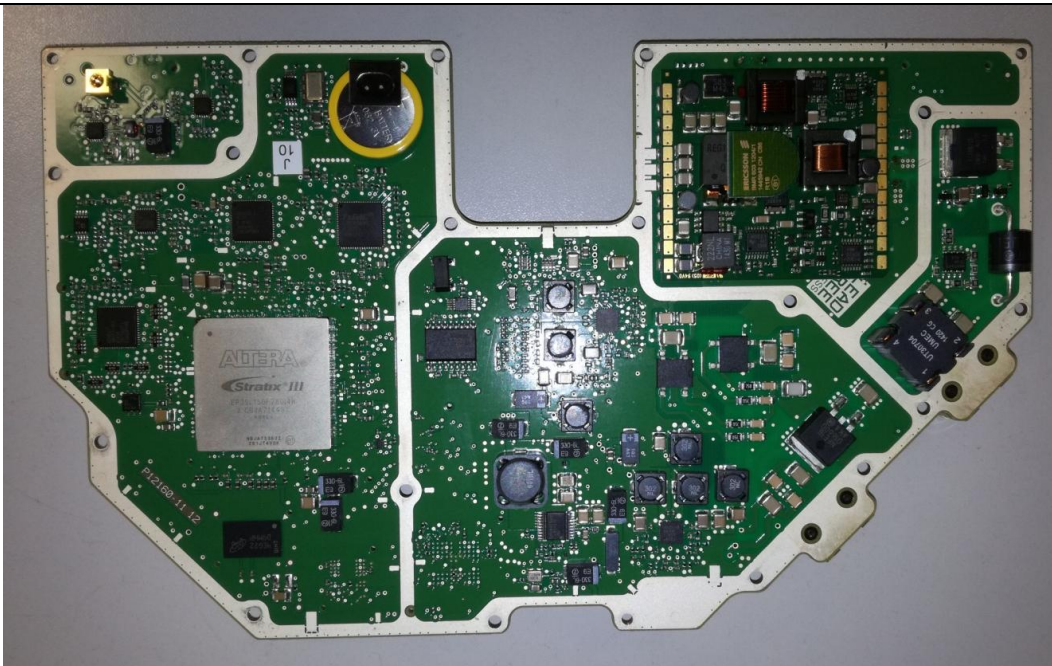
C60226 BOTTOM VIEW (GB9732-04 and GB9733-04)
