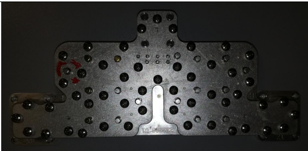
BRANCHING FILTER TOP VIEW (valid for all models)
