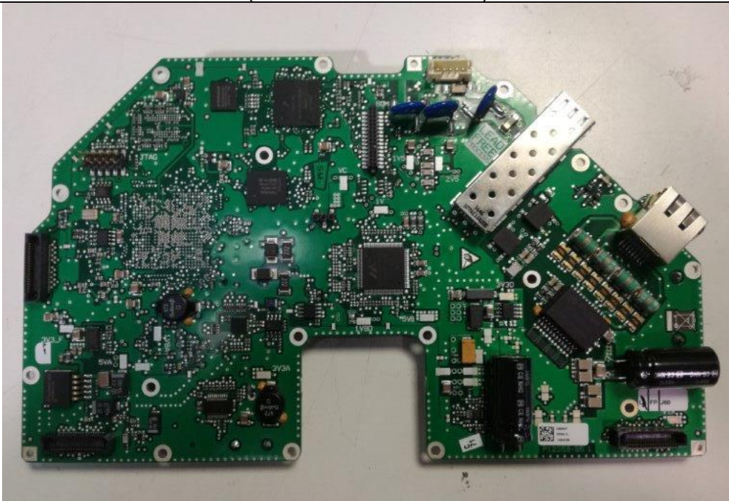
C60447 TOP VIEW (GB7732-04 and GB7733-04)
