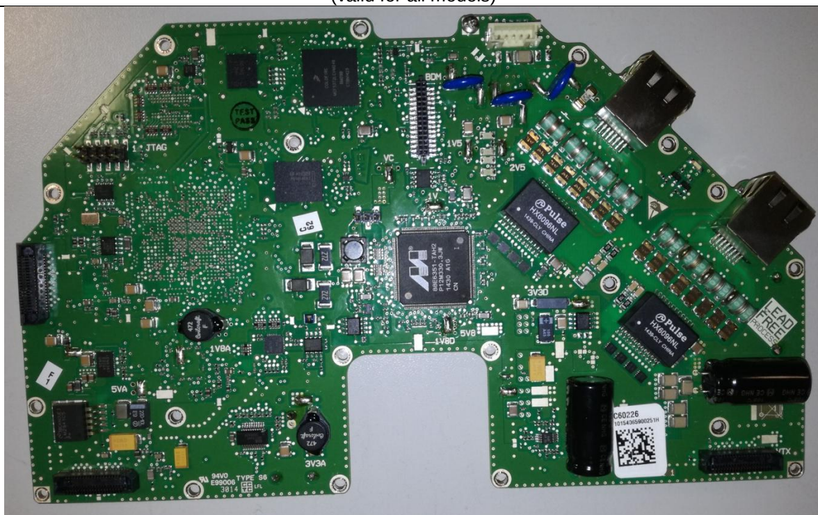
C60226 TOP VIEW (GB9732-04 and GB9733-04)
