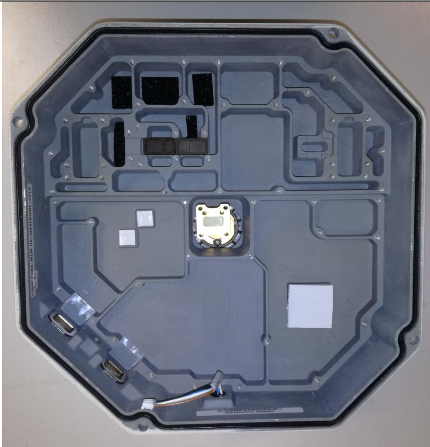
ALFOplus24 METALLIC ENCLOSURE TOP VIEW (valid for all models)
