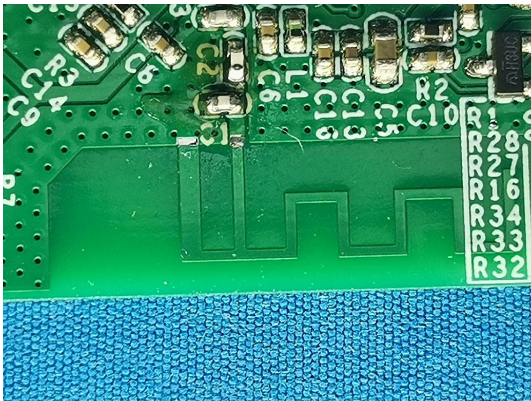
WiFi Antenna
