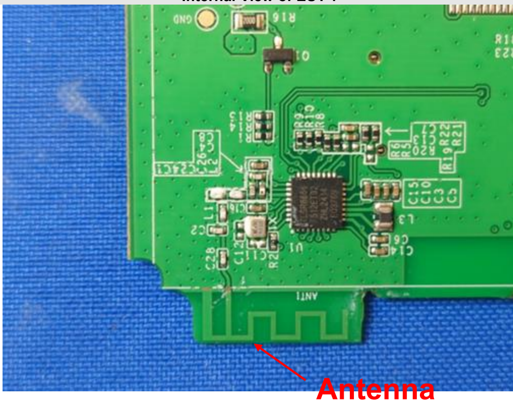
Internal View of EUT-8
