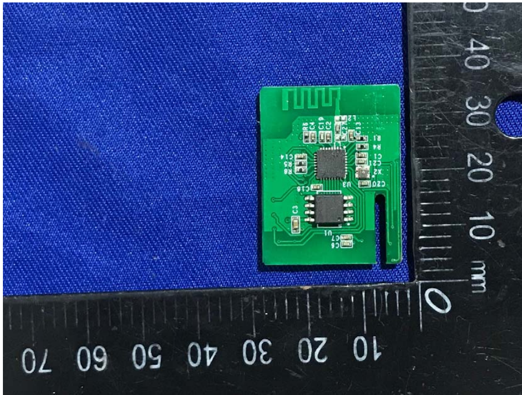
RF board
