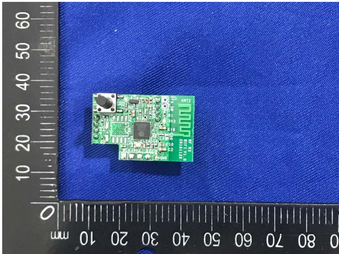
Wi-Fi Chip
