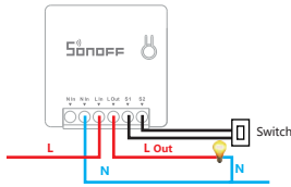
4.2 The wiring diagram to connect the light.
