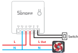
4.1 The wiring diagram to connect the electrical appliance.
