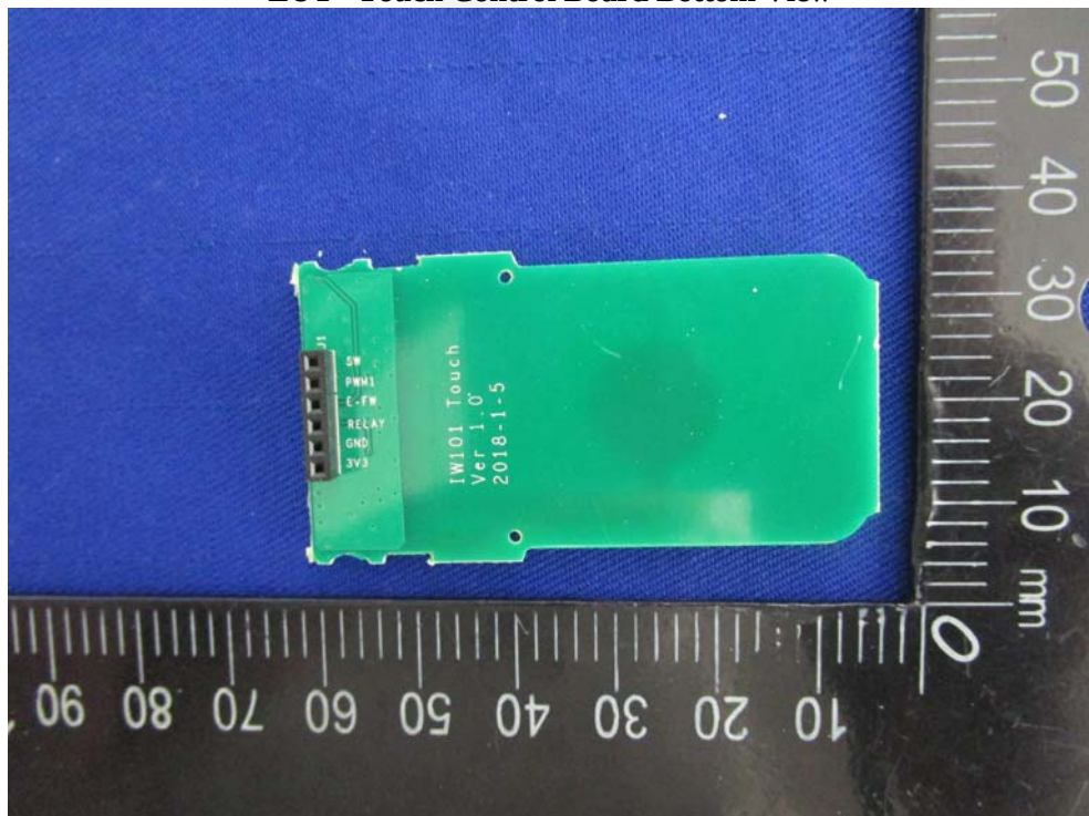
EUT –Touch Control Board Bottom View
