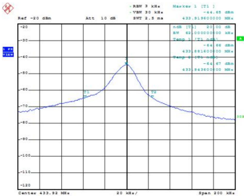
20dBc Bandwidth Test Plot
