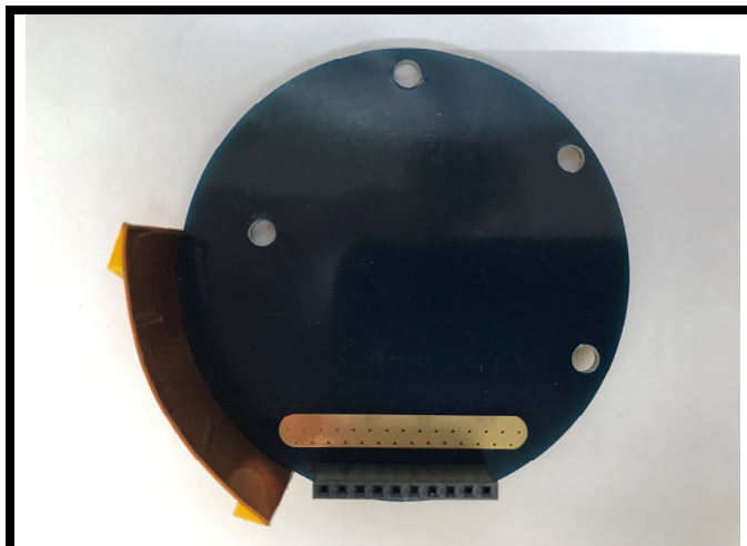
Internal Photo # 3 – Shield PCB Bottom Side
