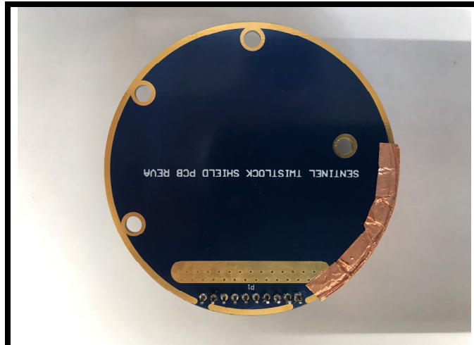
Internal Photo # 4 – Shield PCB Top Side
