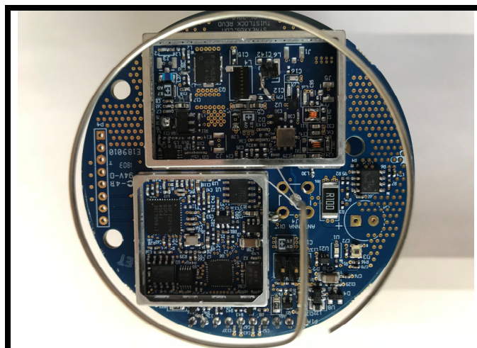
Internal Photo # 6 –Upper PCB Top Side Shield Open
