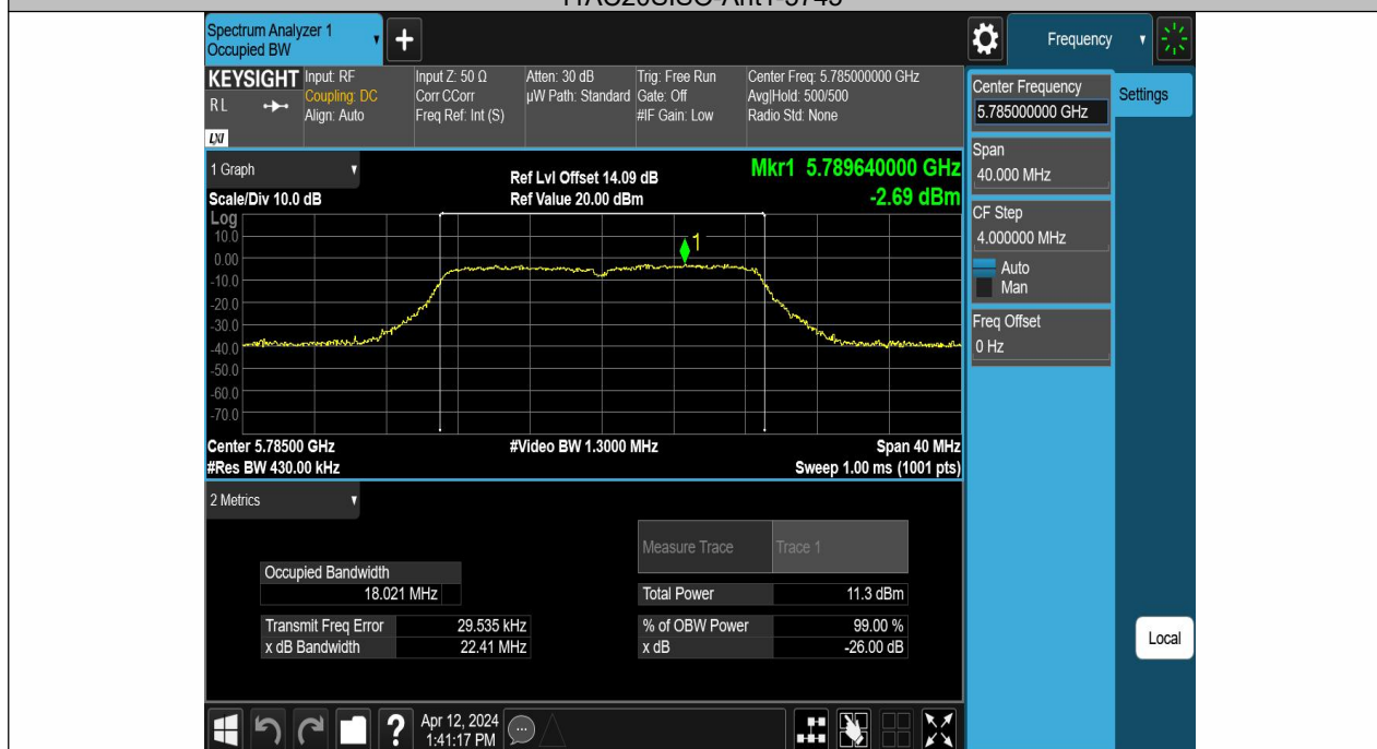
11AC20SISO-Ant1-5785
