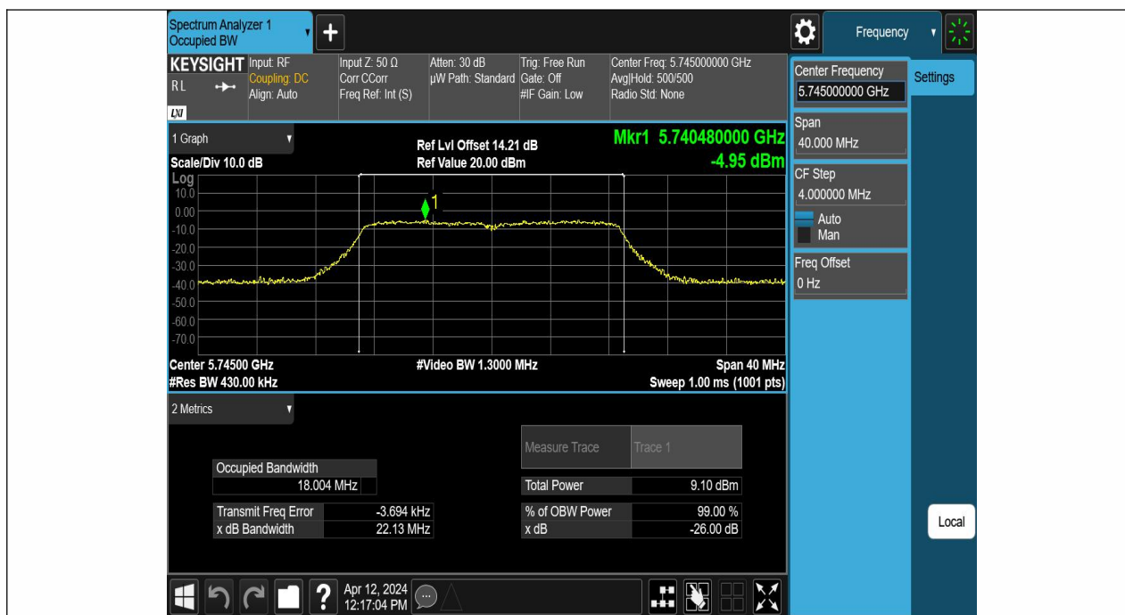
11AC20SISO-Ant1-5745
