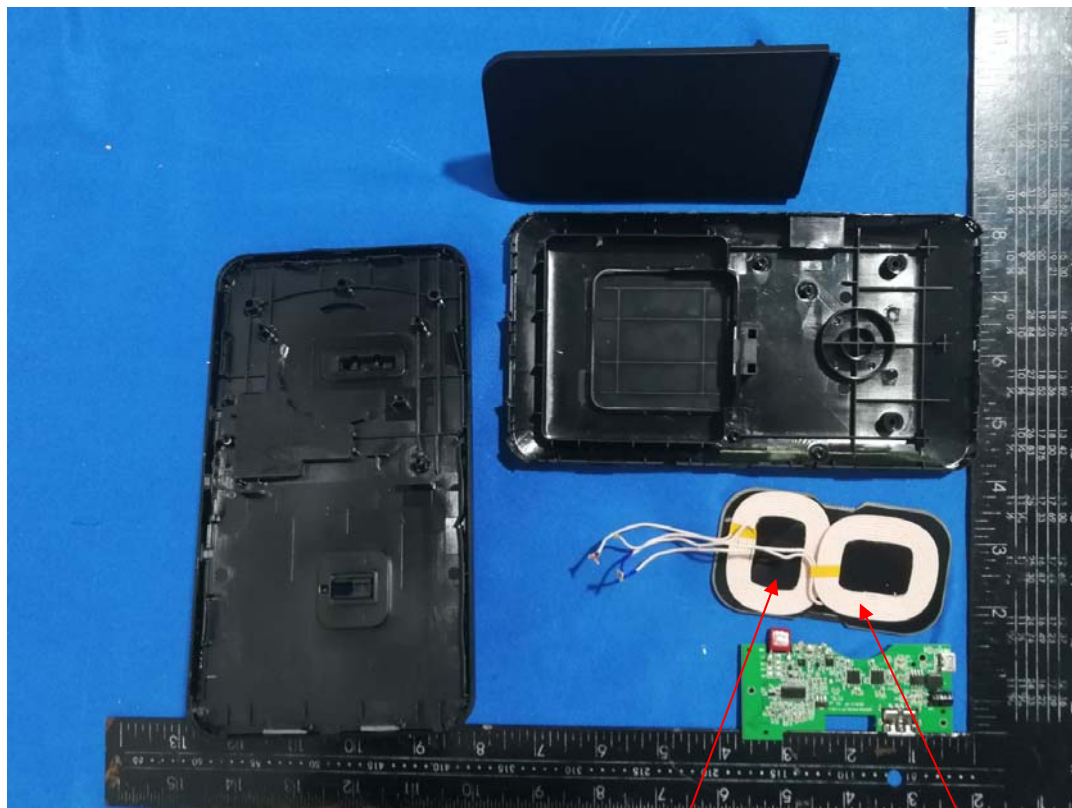
Bottom Coil
