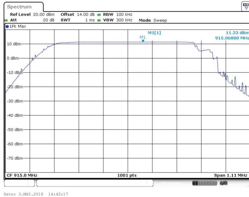
PSD 100kHz Plot
