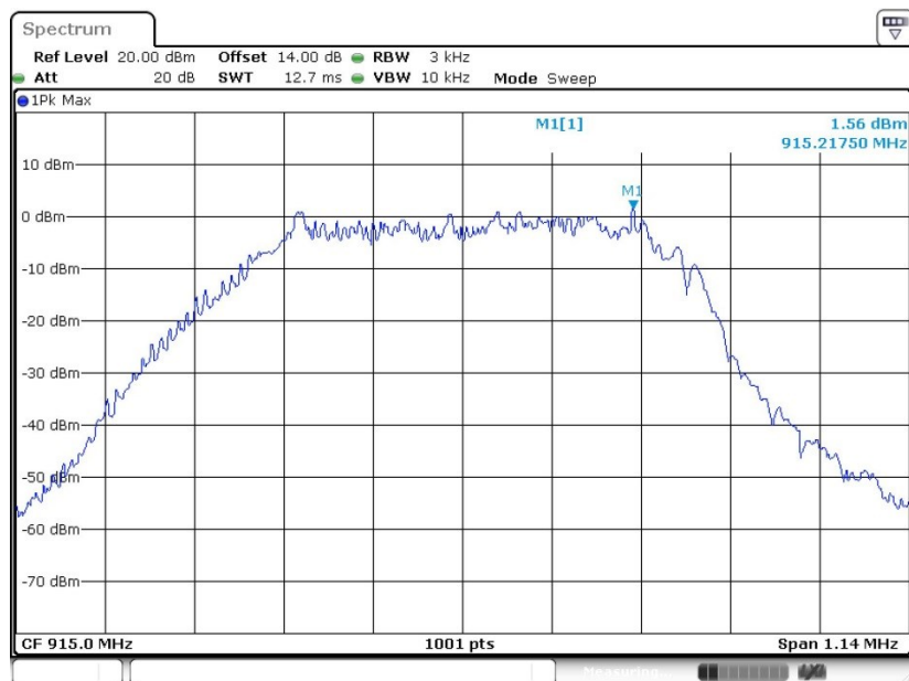
PSD 3kHz Plot
