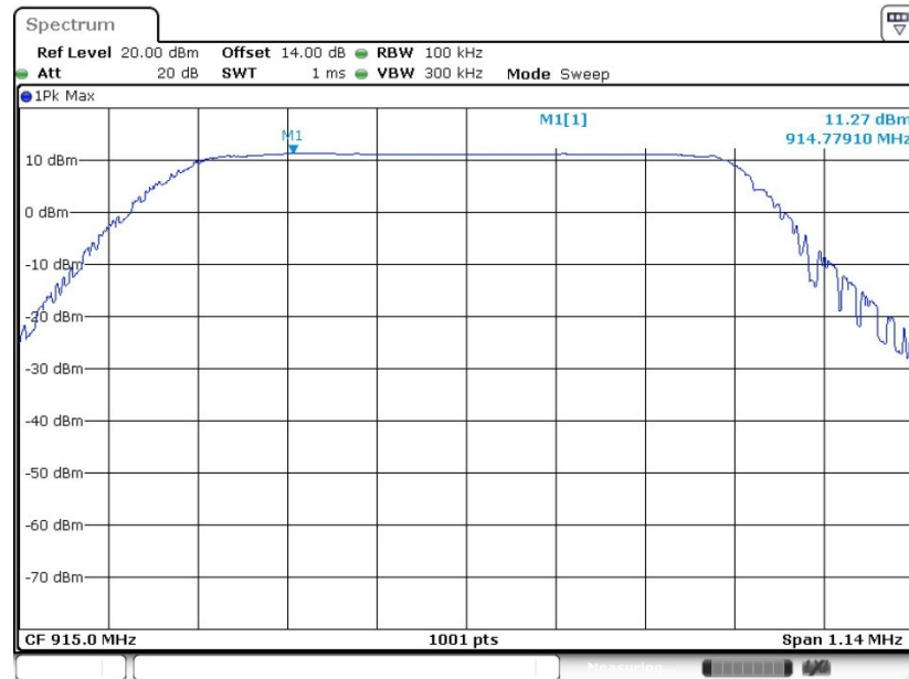
PSD 100kHz Plot
