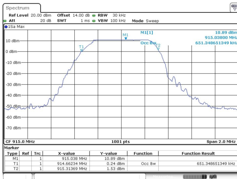
99% Bandwidth Plot
