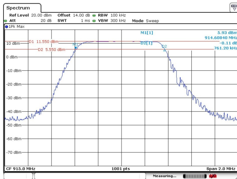
6 dB Bandwidth Plot
