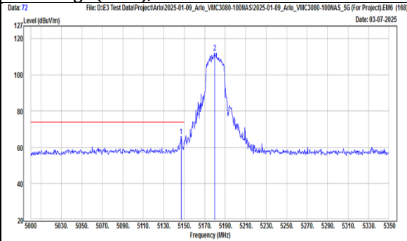
TX, 802.11n(HT20) (Ch 36) Band Edge (Peak), Horizontal
