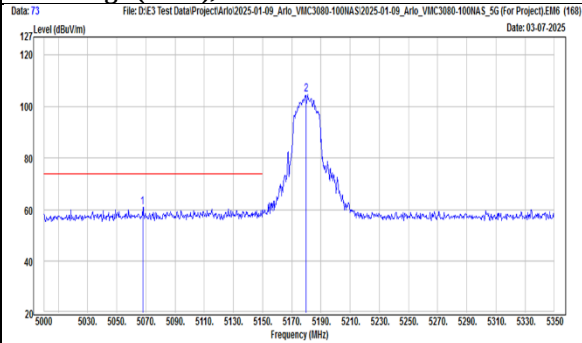
TX, 802.11n(HT20) (Ch 36) Band Edge (Peak), Vertical
