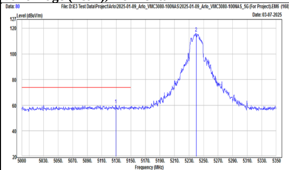
TX, 802.11n(HT20) (Ch 48) Band Edge (Peak), Horizontal
