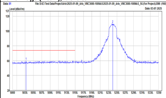
TX, 802.11n(HT20) (Ch 48) Band Edge (Peak), Vertical
