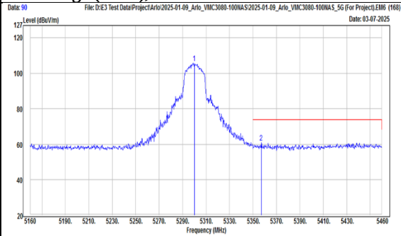
TX, 802.11n(HT20) (Ch 60) Band Edge (Peak), Vertical
