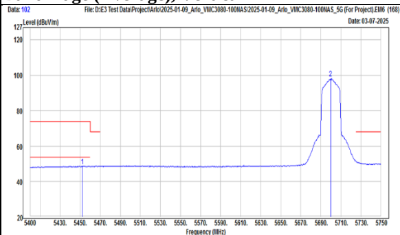
TX, 802.11n(HT20) (Ch 140) Band Edge (Peak), Vertical
