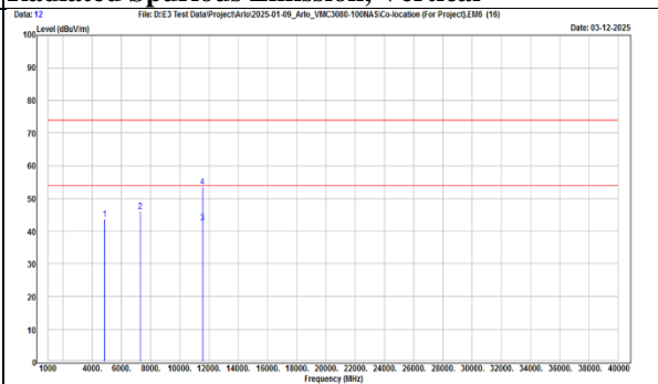
TX, 5G 802.11a (Ch157) & BT-LE (Ch 19) Radiated Spurious Emission, Vertical
