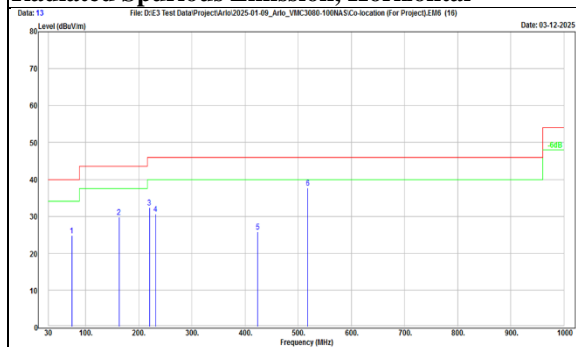
TX, 2.4G 802.11b (Ch6) & BT-LE (Ch 19) Radiated Spurious Emission, Horizontal
