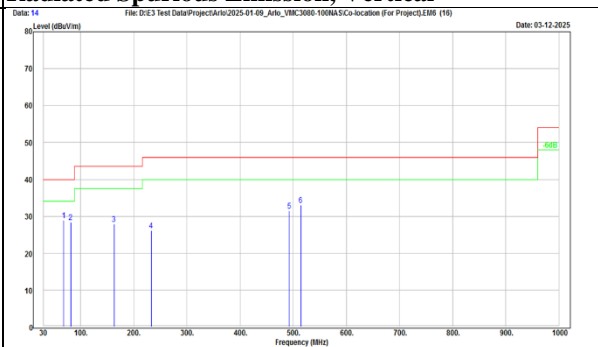
TX, 2.4G 802.11b (Ch6) & BT-LE (Ch 19) Radiated Spurious Emission, Vertical
