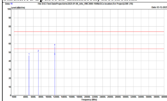
TX, 5G 802.11a (Ch157) & BT-LE (Ch 19) Radiated Spurious Emission, Horizontal
