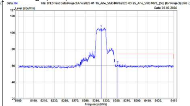
TX, 802.11n(HT20) (Ch 64) Band Edge (Peak), Vertical
