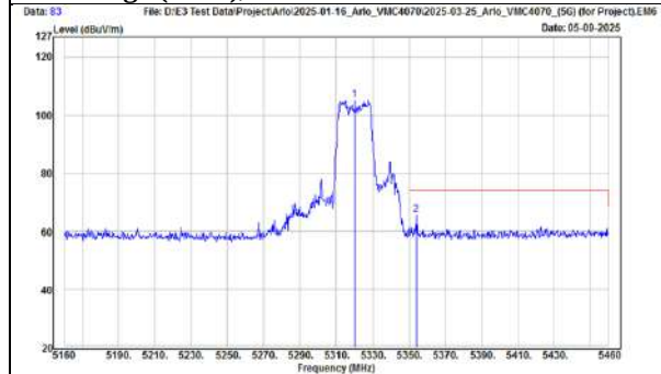
TX, 802.11n(HT20) (Ch 64) Band Edge (Peak), Horizontal
