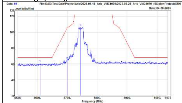
TX, 802.11a (Ch 149) Band Edge (Peak), Horizontal
