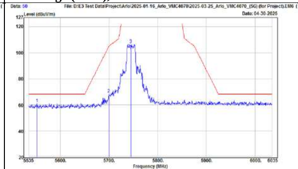
TX, 802.11a (Ch 149) Band Edge (Peak), Vertical
