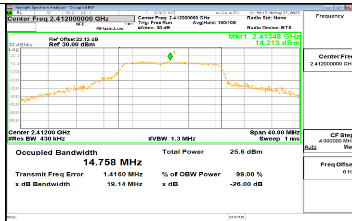
11N20SISO Ant1 2412
