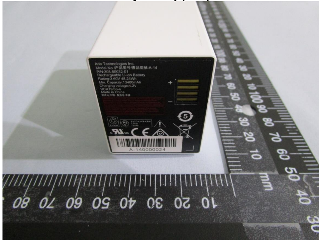
Accessory: Battery (A-14) Pic 5
