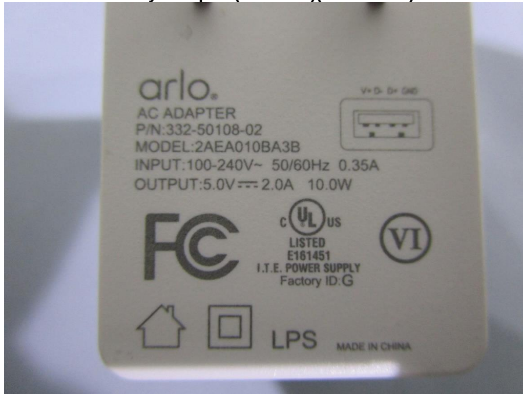
Accessory: Adapter (2AEA010)(Not for Sell) Pic 5
