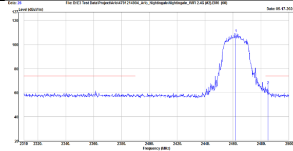
2.4G WiFi (#2)-TX, 802.11n(HT20) (Ch 11) Band Edge (Peak), Horizontal
