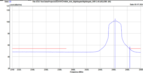
2.4G WiFi (#2)-TX, 802.11n(HT20) (Ch 11) Band Edge (Peak), Vertical
