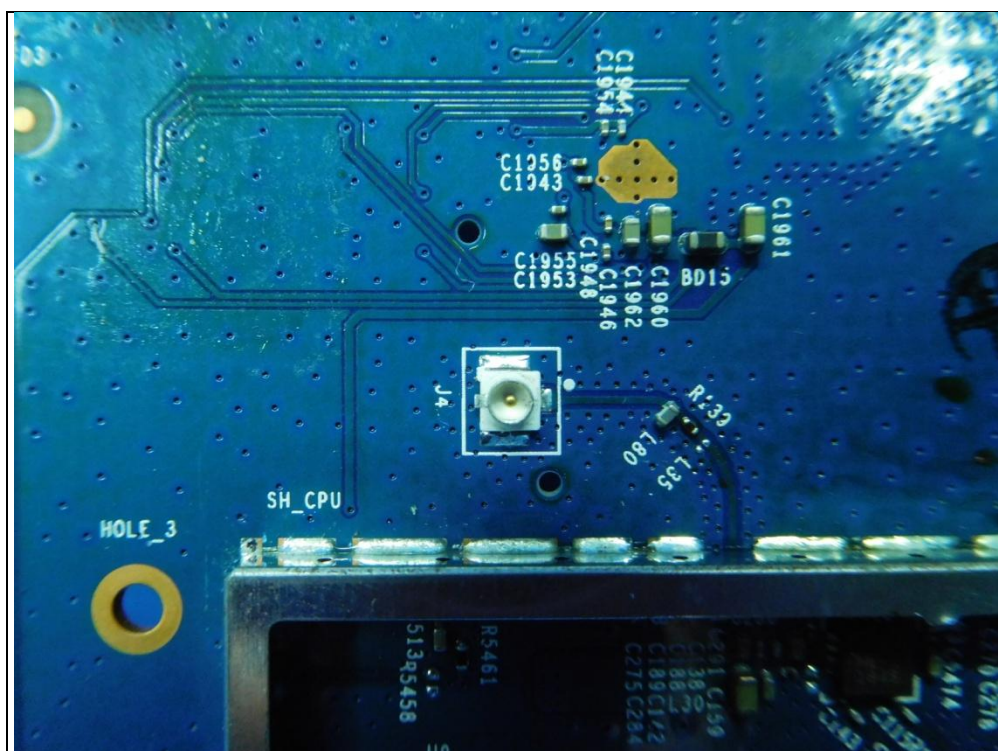
WLAN Antenna 1
