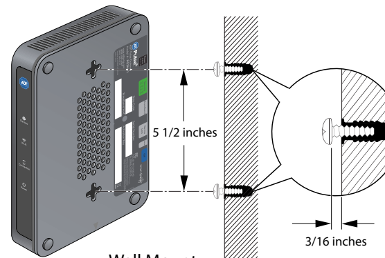
Wall Mount
