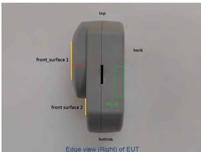
Fig.13 Edges/surfaces definition
