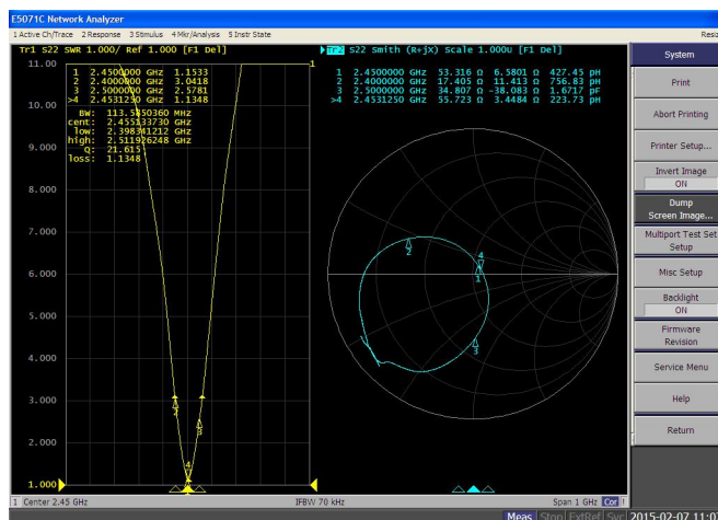
Fig.1 驻波比 VSWR
