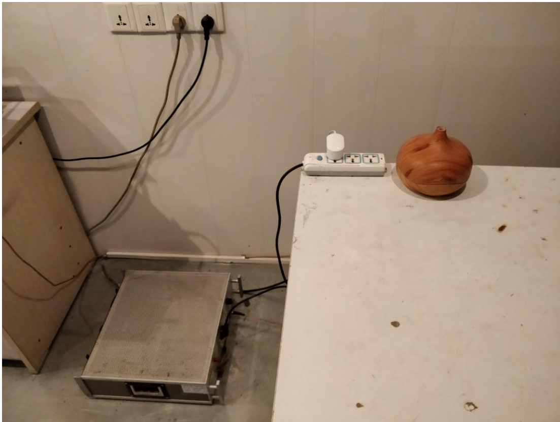
Conducted Emission (adapter: HN BG240060WU)
