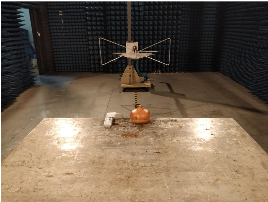
Radiated Emission (adapter: HNBG240060WU)
