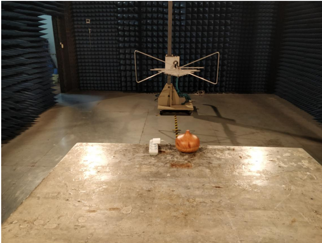
Radiated Emission (adapter:SK02T-2400060U)
