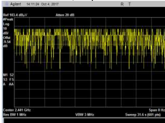
Plot 16. Dwell Time, DH5 burst per period = 129
