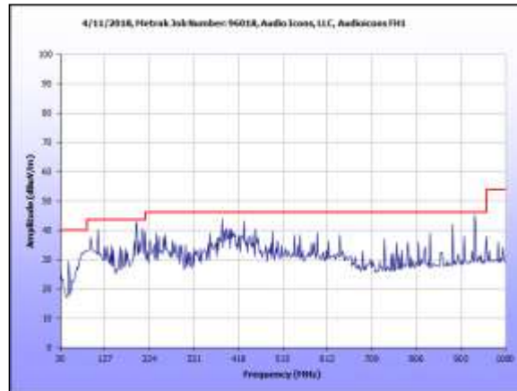
Plot 72. Radiated Emissions, 15.209 Low Channel
