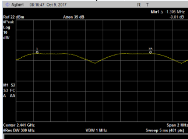
Plot 33. Channel Separation, 2441, DH1
