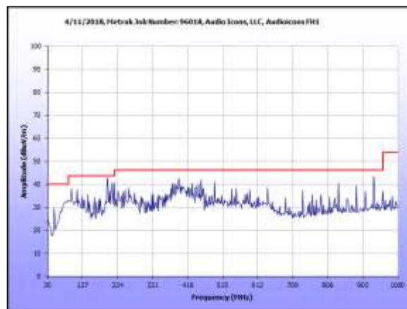
Plot 74. Radiated Emissions, 15.209 High Channel
