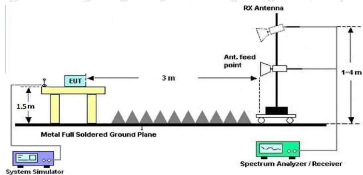
Figure 3. Above 1 GHz
