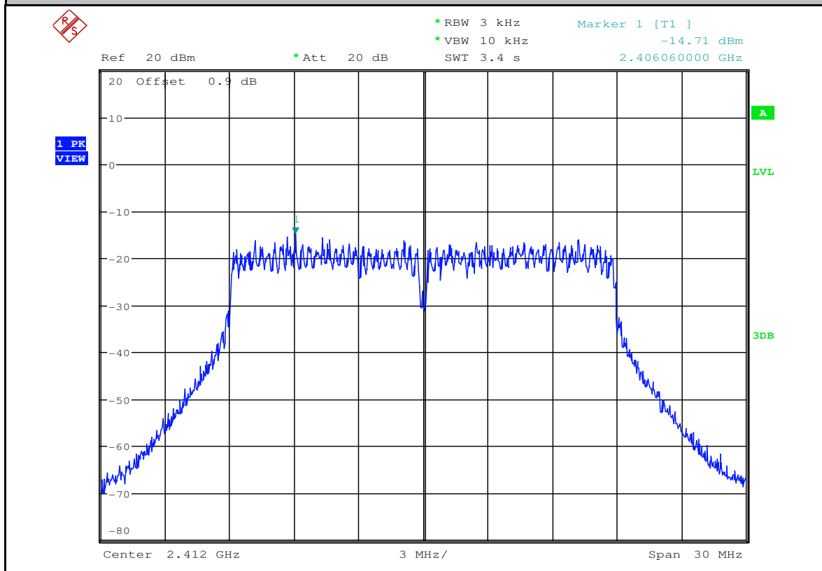
Maximum Peak power spectral density_11N20SISO_2412_Ant2
