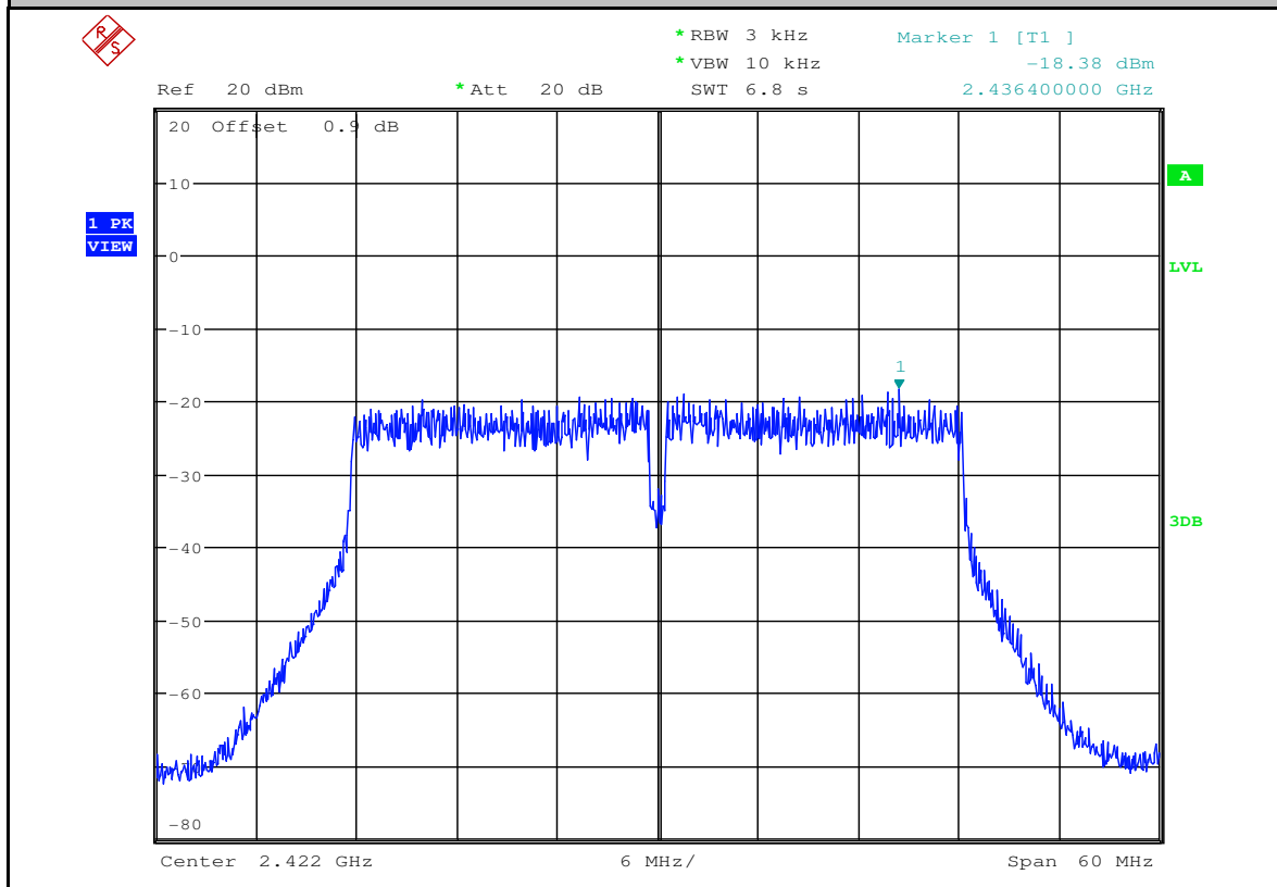
Maximum Peak power spectral density_11N40SISO_2422_Ant2
