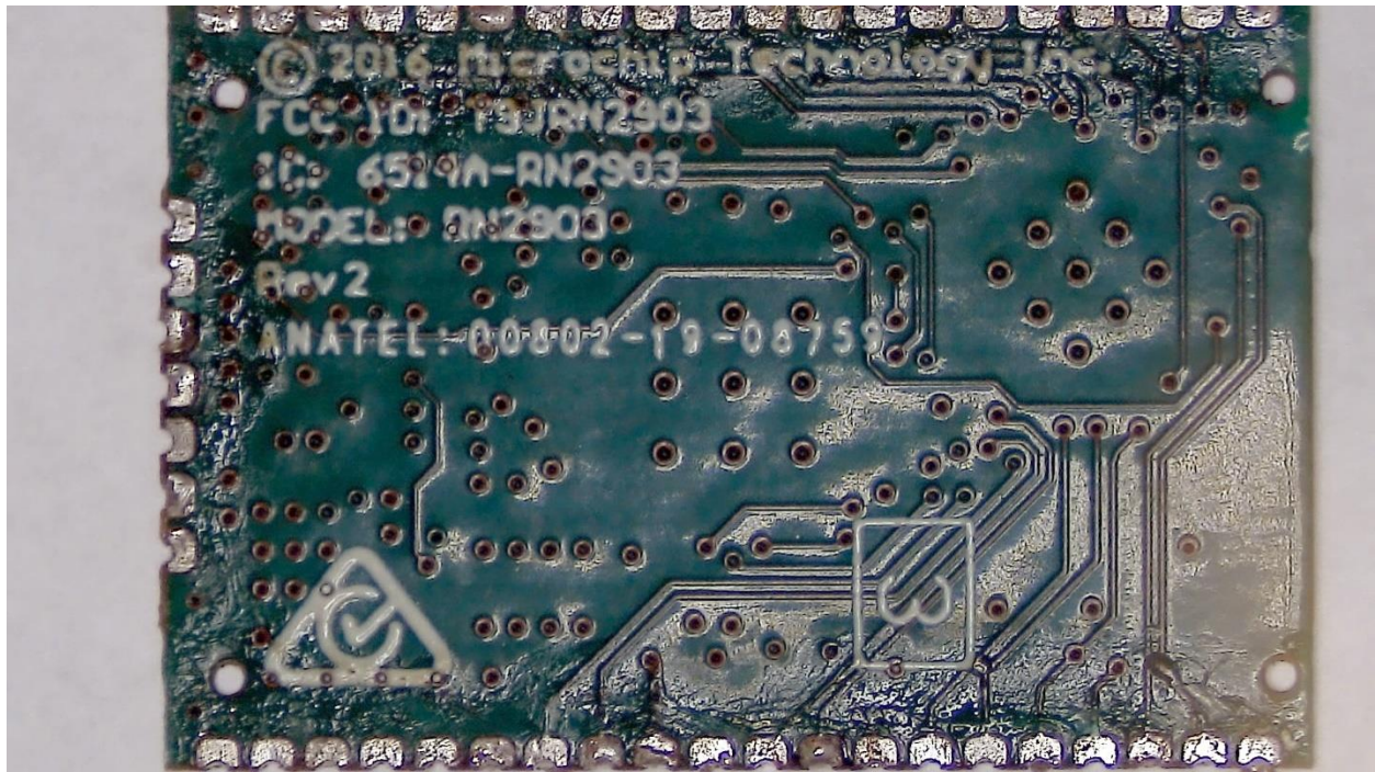
Integrated RF Module RN2903 bottom side with FCC / ISED ID's
