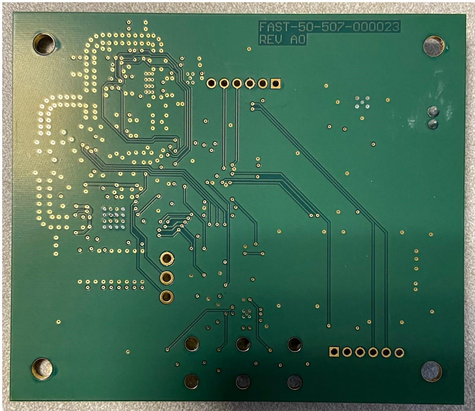
PCB bottom side
