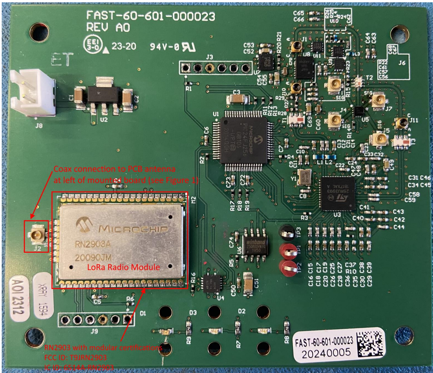
PCB top side
