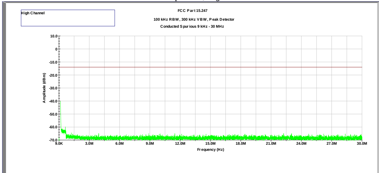
Plot 4.3 Transmitter Spurious, High Channel
