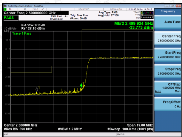
LCH_QPSK_100RB#0
