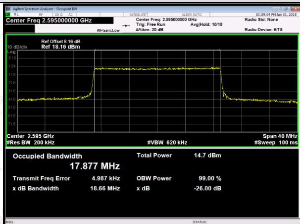
MCH_16QAM_100RB#0
