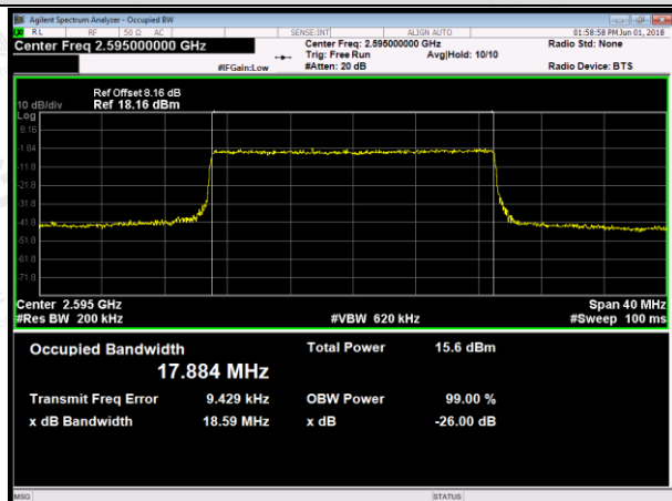
MCH_QPSK_100RB#0
