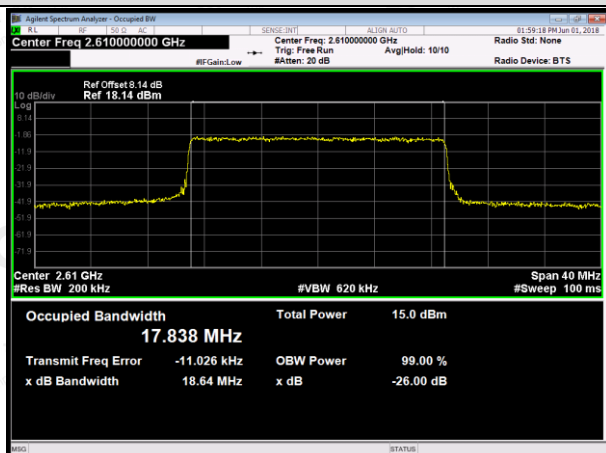
HCH_16QAM_100RB#0
