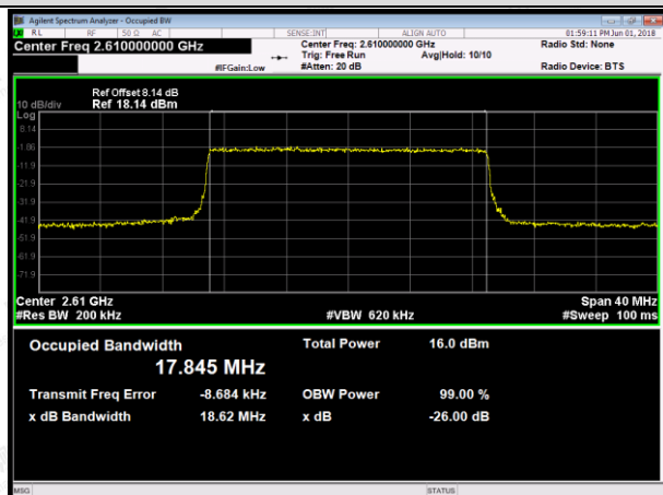
HCH_QPSK_100RB#0
