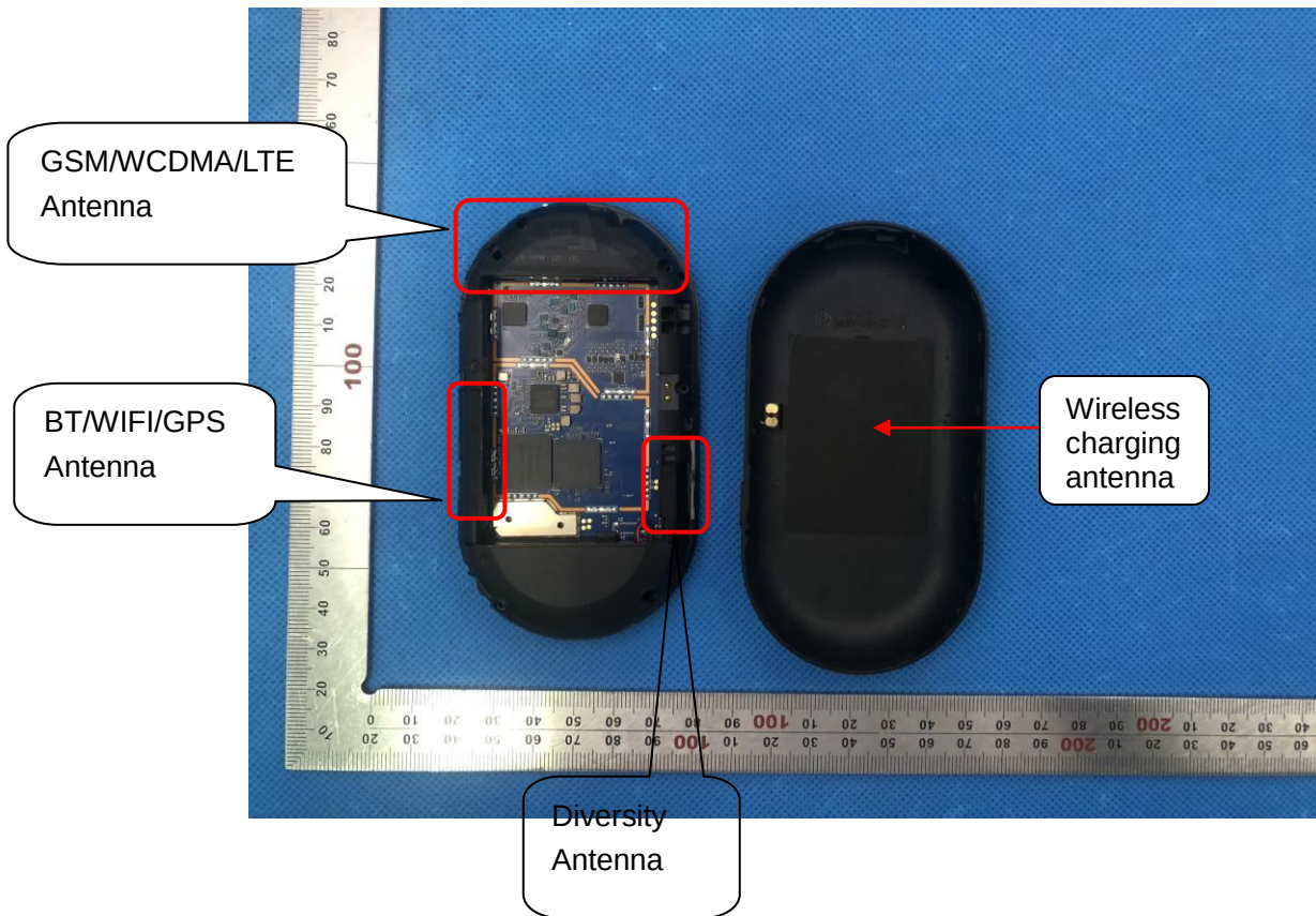
OPEN VIEW OF EUT(FIGURE 2)
