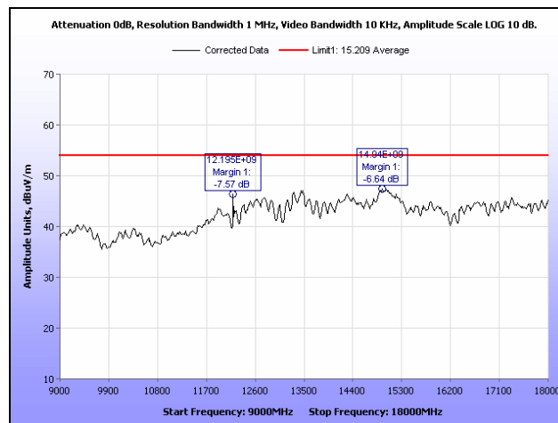
Plot 12. Radiated Spurious Emissions, Mid Channel, 9 GHz – 18 GHz, Average
