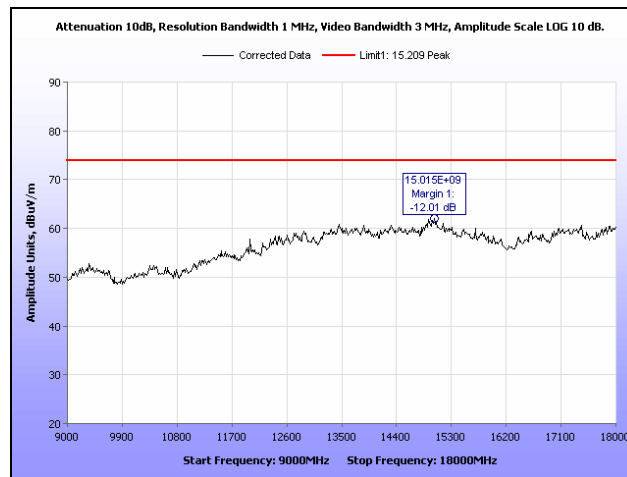
Plot 11. Radiated Spurious Emissions, Low Channel, 9 GHz – 18 GHz, Peak
