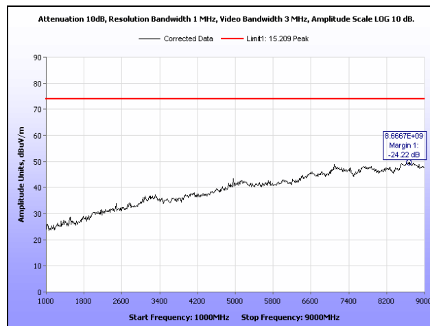
Plot 9. Radiated Spurious Emissions, High Channel, 1 GHz – 9 GHz, Peak
