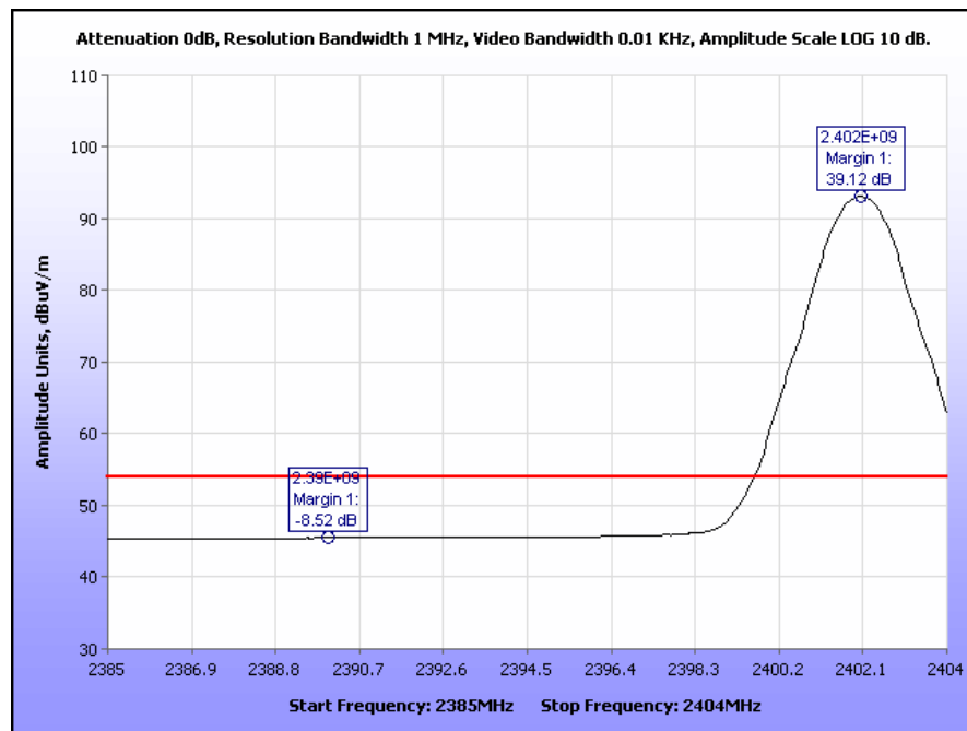
Plot 31. Radiated Restricted Band Edge, Low Channel, 2390 MHz, Average
