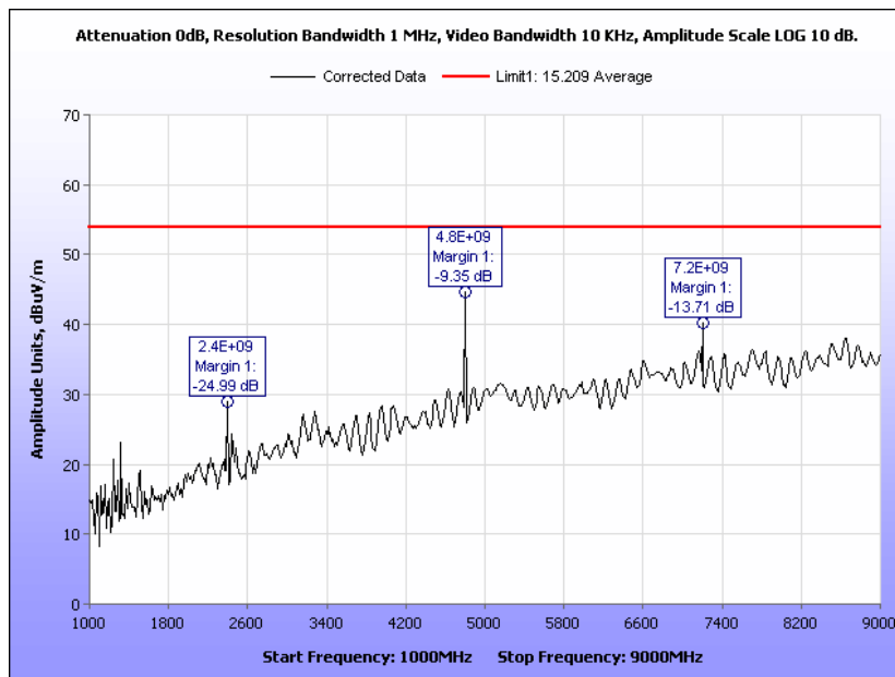
Plot 23. Radiated Spurious Emissions, All Tx Active, 1-9GHz Average
