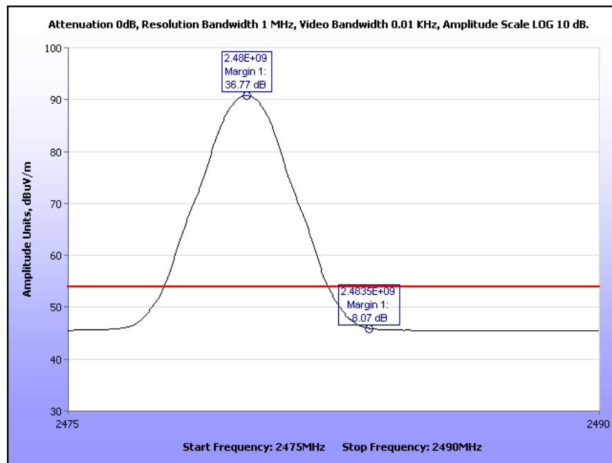
Plot 33. Radiated Restricted Band Edge, High Channel, 2483.5 MHz, Average
