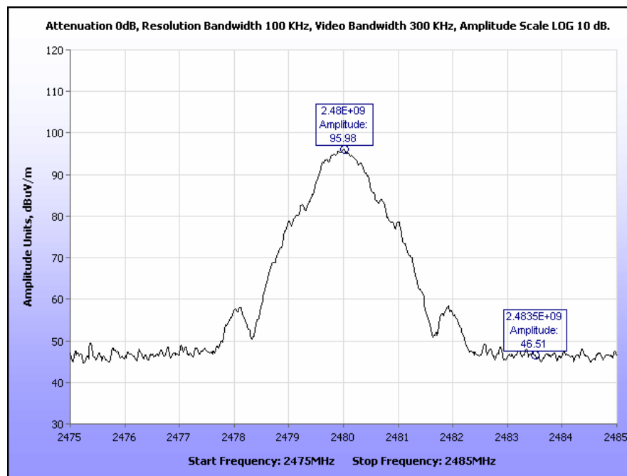
Plot 30. Radiated Restricted Band Edge, High Channel, 20 dBc, 2483.5 MHz
