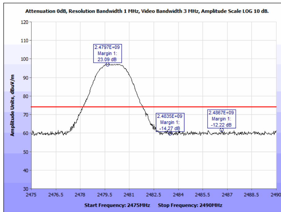
Plot 34. Radiated Restricted Band Edge, High Channel, 2483.5 MHz, Peak
