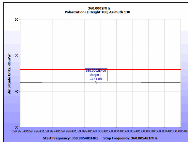
Plot 18. Radiated Spurious Emissions, High Channel, 360.0002 MHz QP
