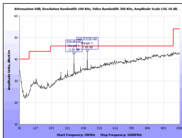
Plot 3. Radiated Spurious Emissions, High Channel, 30 MHz – 1 GHz
