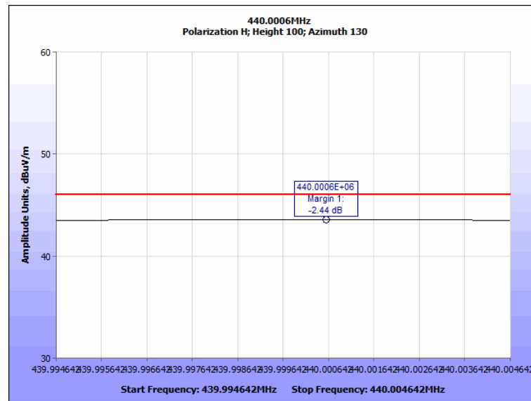
Plot 27. Radiated Spurious Emissions, All Tx Active, 440 MHz QP
