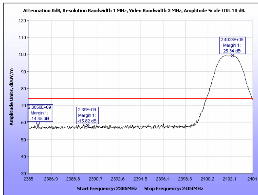
Plot 323. Radiated Restricted Band Edge, Low Channel, 2390 MHz, Peak
