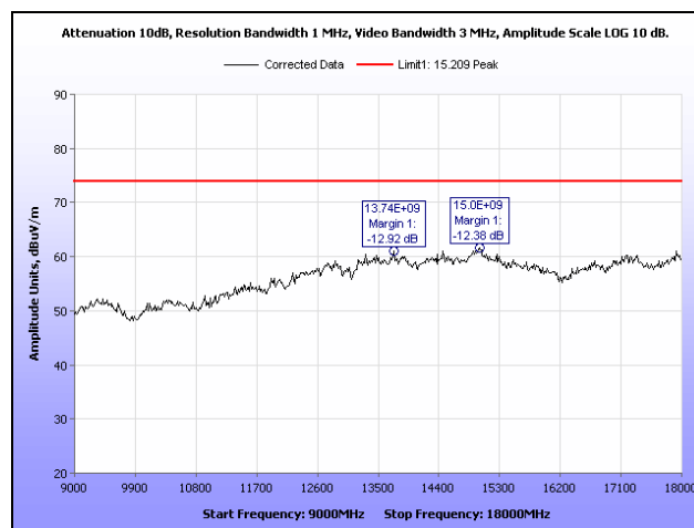
Plot 15. Radiated Spurious Emissions, High Channel, 9 GHz – 18 GHz, Peak
