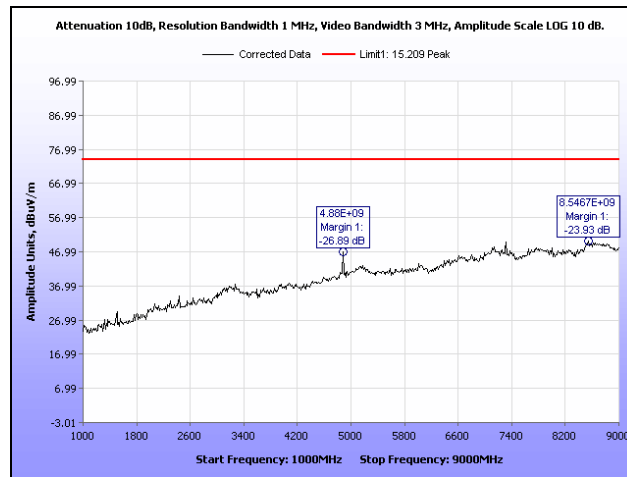
Plot 7. Radiated Spurious Emissions, Mid Channel, 1 GHz – 9 GHz, Peak
