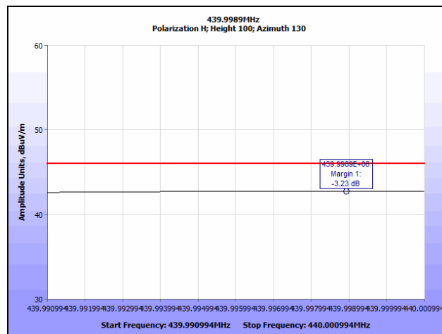
Plot 21. Radiated Spurious Emissions, High Channel, 439.9989 MHz QP
