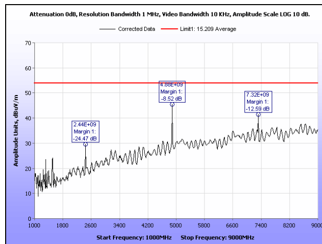
Plot 6. Radiated Spurious Emissions, Mid Channel, 1 GHz – 9 GHz, Average
