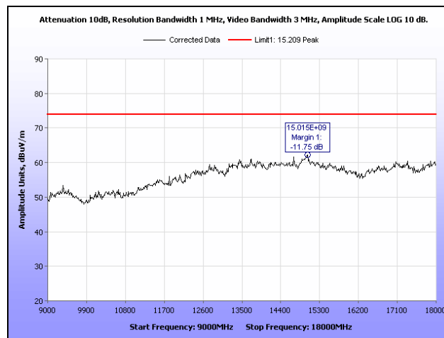
Plot 13. Radiated Spurious Emissions, Mid Channel, 9 GHz – 18 GHz, Peak
