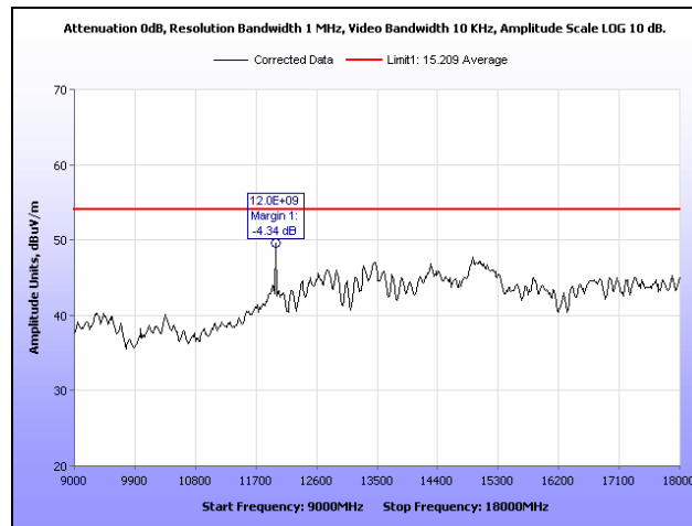
Plot 10. Radiated Spurious Emissions, Low Channel, 9 GHz – 18 GHz, Average
