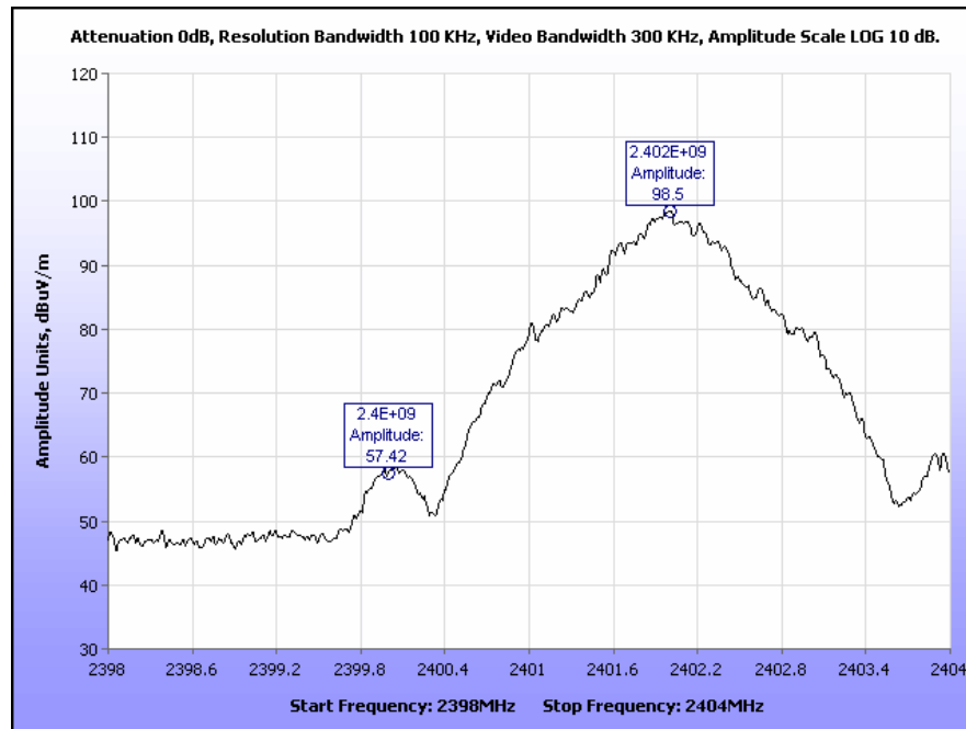
Plot 29. Radiated Restricted Band Edge, Low Channel, 20 dBc, 2400 MHz
