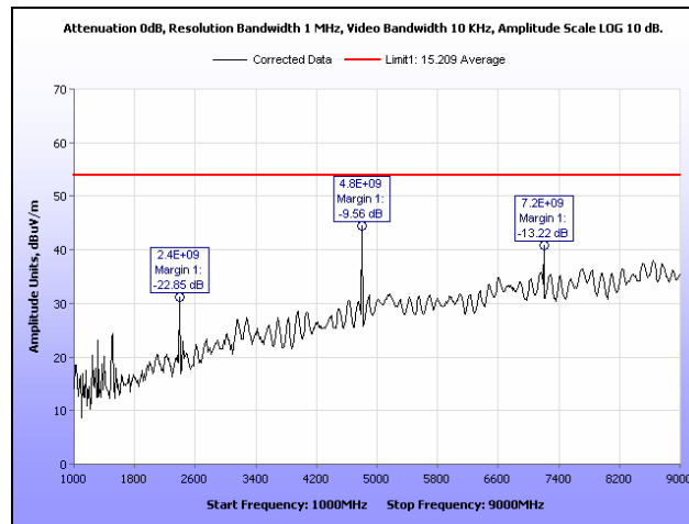
Plot 4. Radiated Spurious Emissions, Low Channel, 1 GHz – 9 GHz, Average
