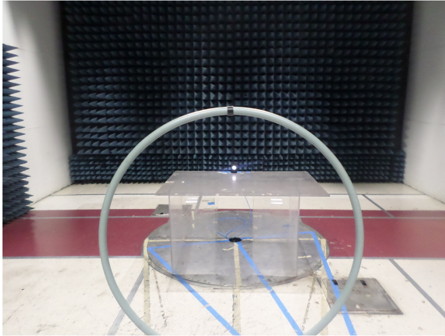
Photograph 1. Spurious Emissions, Test Setup, 9 kHz – 150 kHz, 0°
