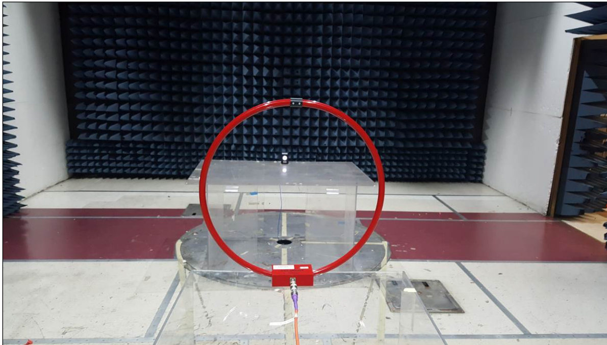
Photograph 2. Spurious Emissions, Test Setup, 150 kHz – 30 MHz, 0°
