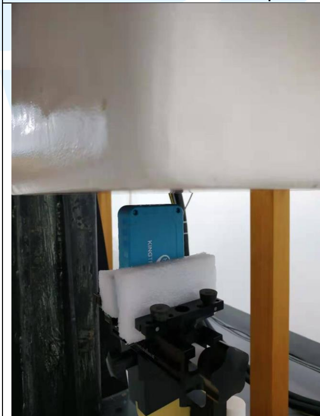
Left Side of EUT with 1.0 cm Gap
