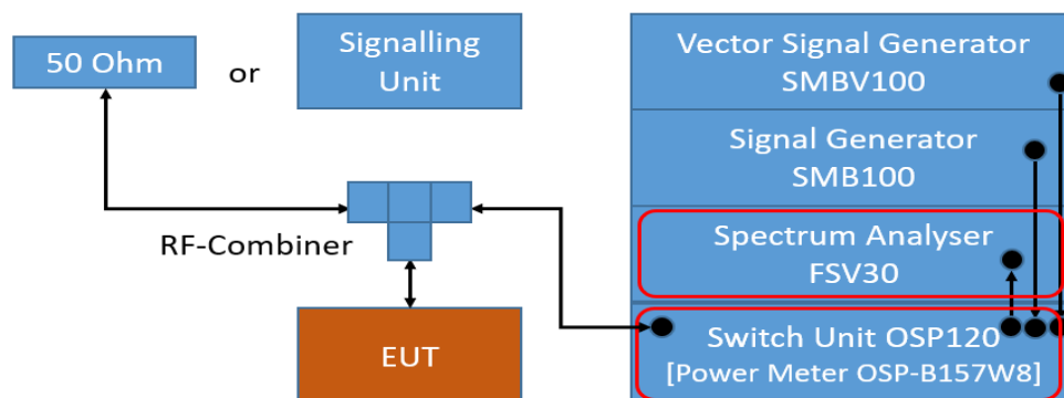
TS8997; Output Power
