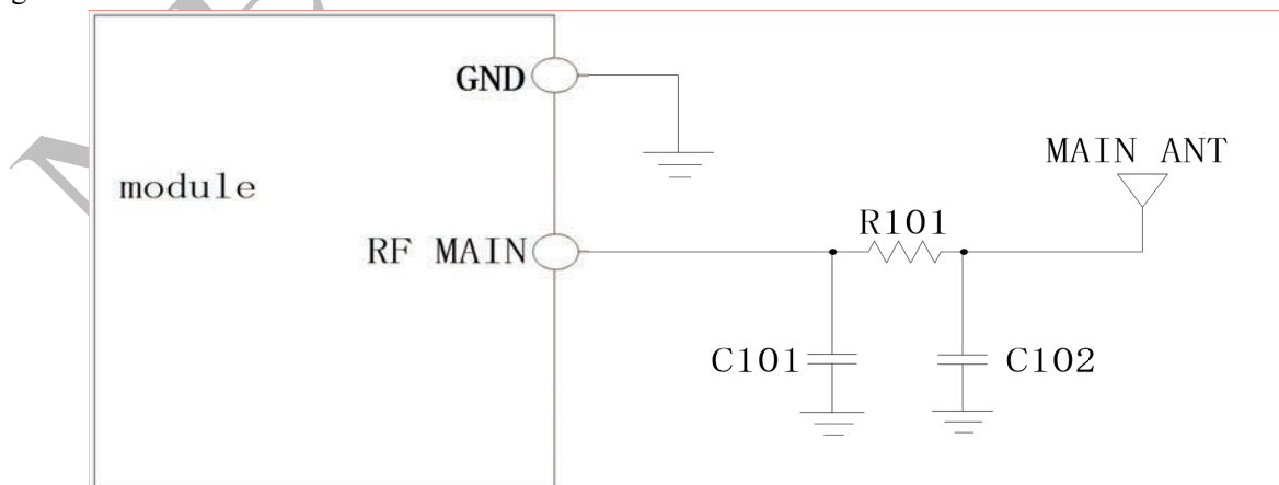
Figure 4.28: ANT_0/1/2/3 antenna interface simplified connection circuit
