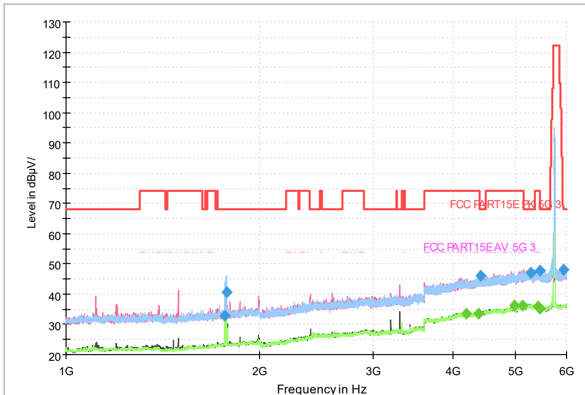
Fig.279 Radiated emission: 802.11n(20M),CH149, 1GHz-6GHz
