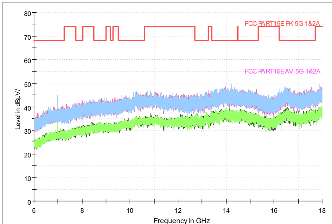
Fig.306 Radiated emission: 802.11ac(20M),CH40, 6GHz-18GHz
