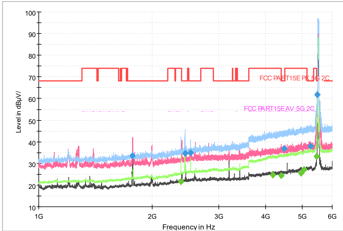
Fig.293 Radiated emission: 802.11n(40M),CH102, 1GHz-6GHz
