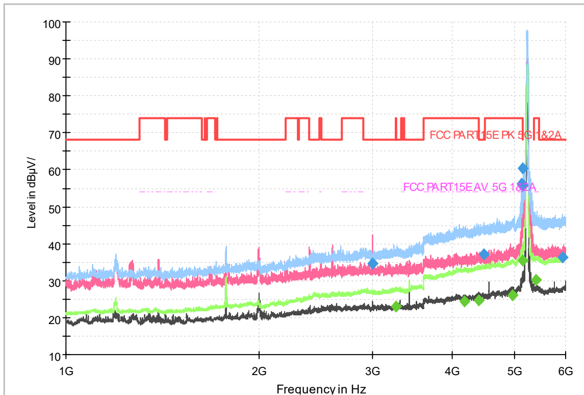
Fig.287 Radiated emission: 802.11n(40M),CH46, 1GHz-6GHz
