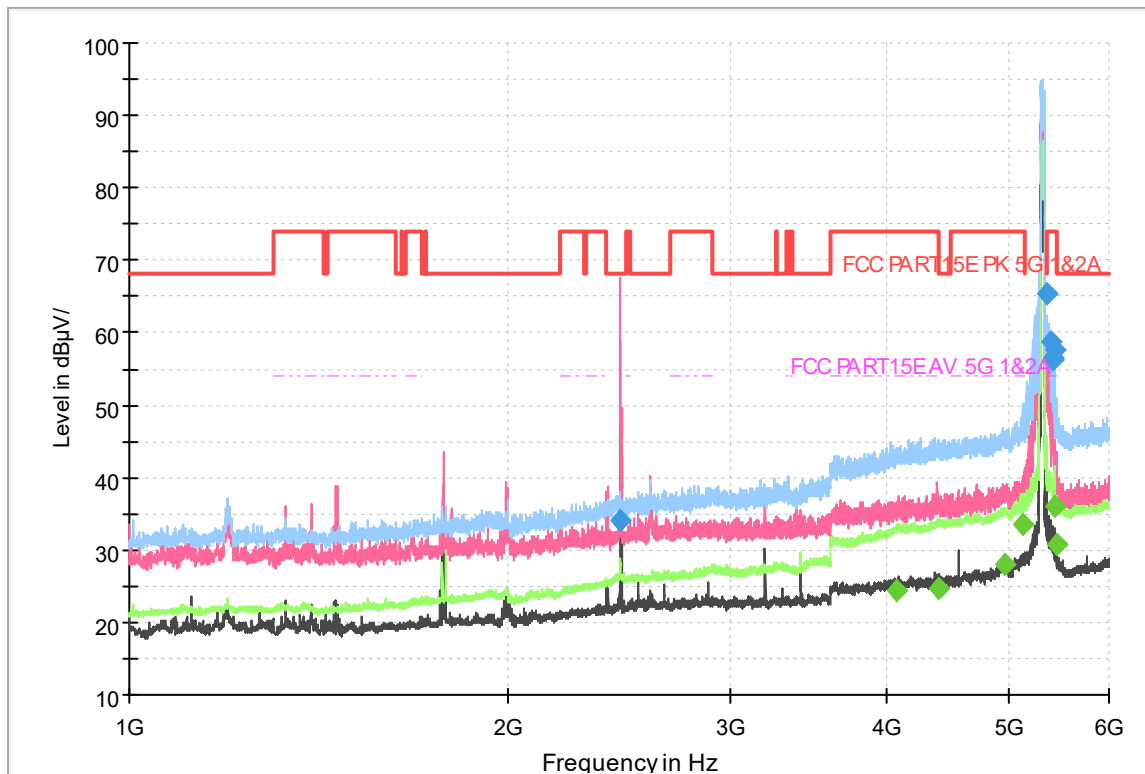
Fig.291 Radiated emission: 802.11n(40M),CH62, 1GHz-6GHz
