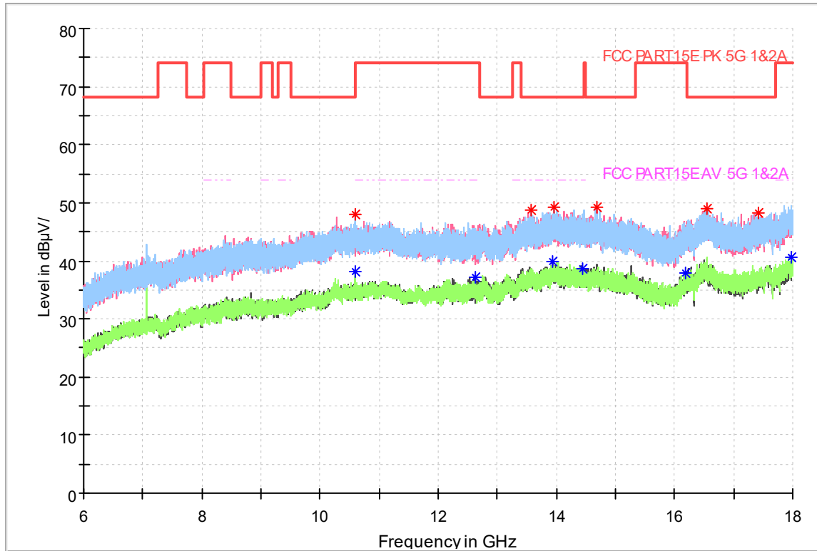
Fig.290 Radiated emission: 802.11n(40M),CH54, 6GHz-18GHz
