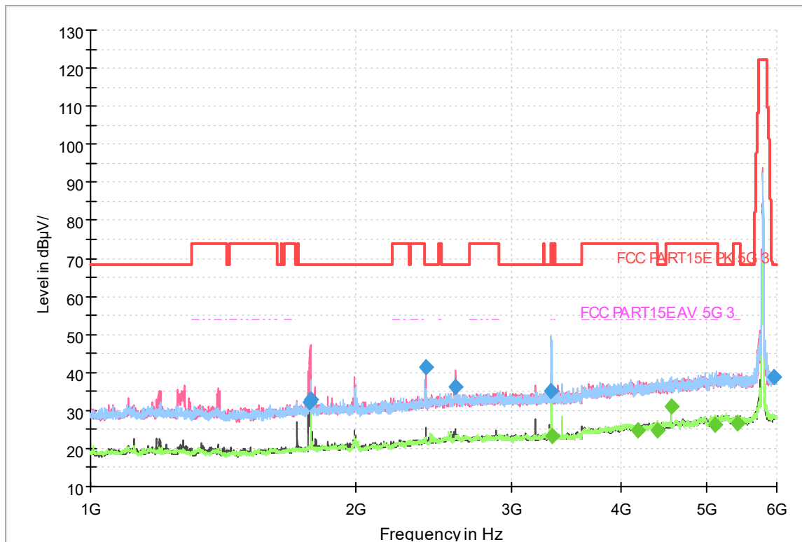
Fig.281 Radiated emission: 802.11n(20M),CH157, 1GHz-6GHz
