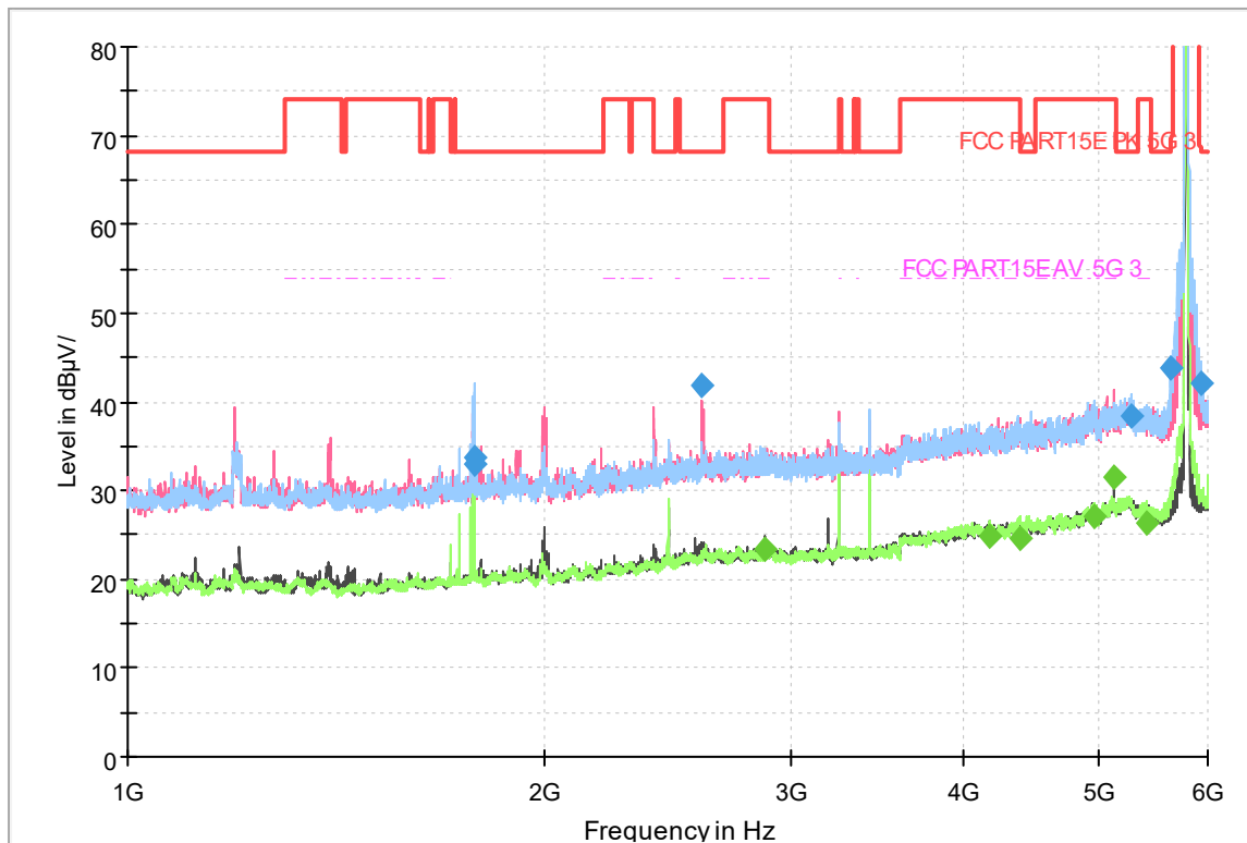
Fig.301 Radiated emission: 802.11n(40M),CH159, 1GHz-6GHz
