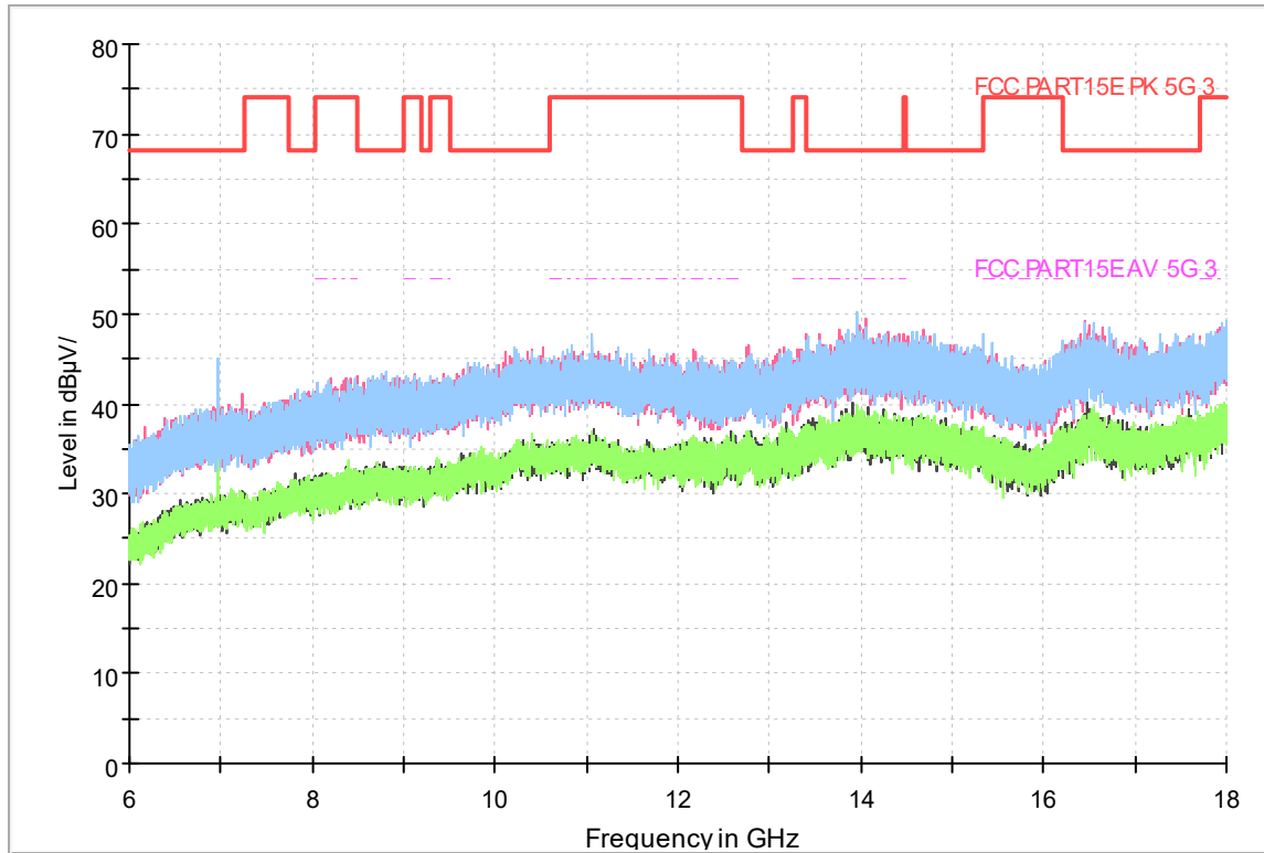
Fig.282 Radiated emission: 802.11n(20M),CH157, 6GHz-18GHz
