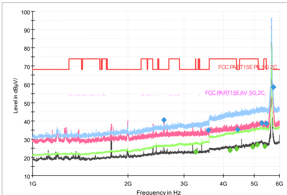
Fig.297 Radiated emission: 802.11n(40M),CH134, 1GHz-6GHz
