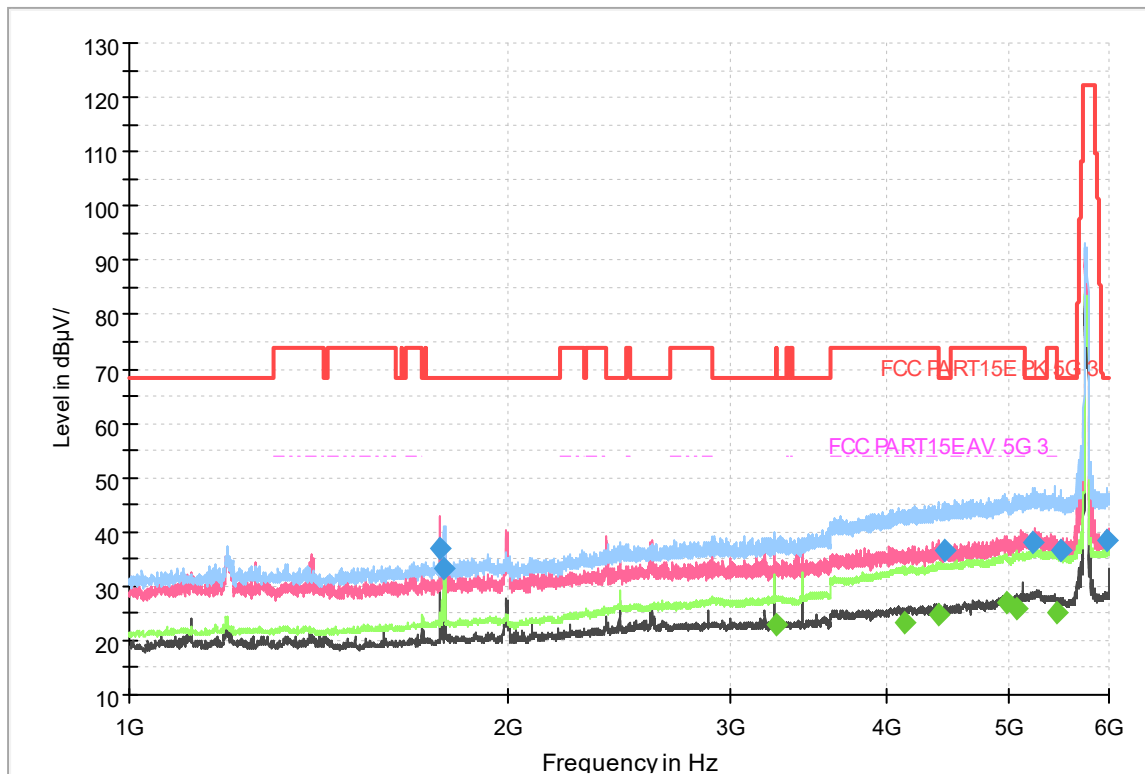
Fig.299 Radiated emission: 802.11n(40M),CH151, 1GHz-6GHz
