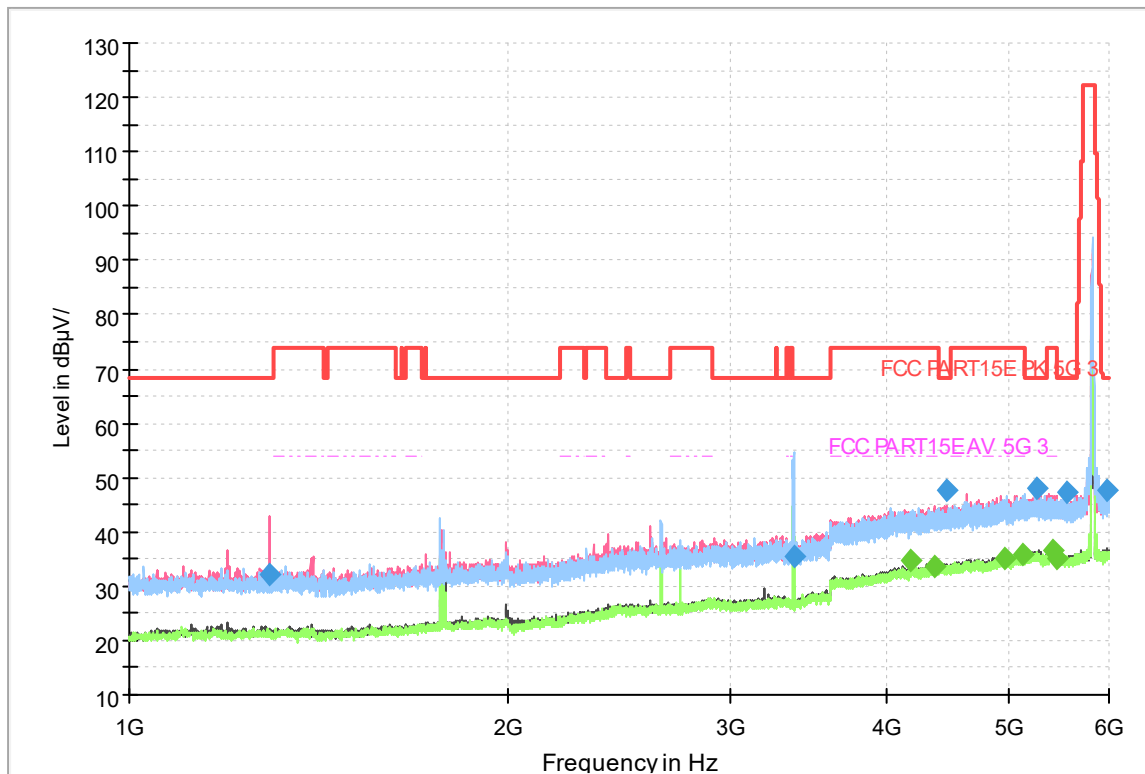
Fig.283 Radiated emission: 802.11n(20M),CH165, 1GHz-6GHz
