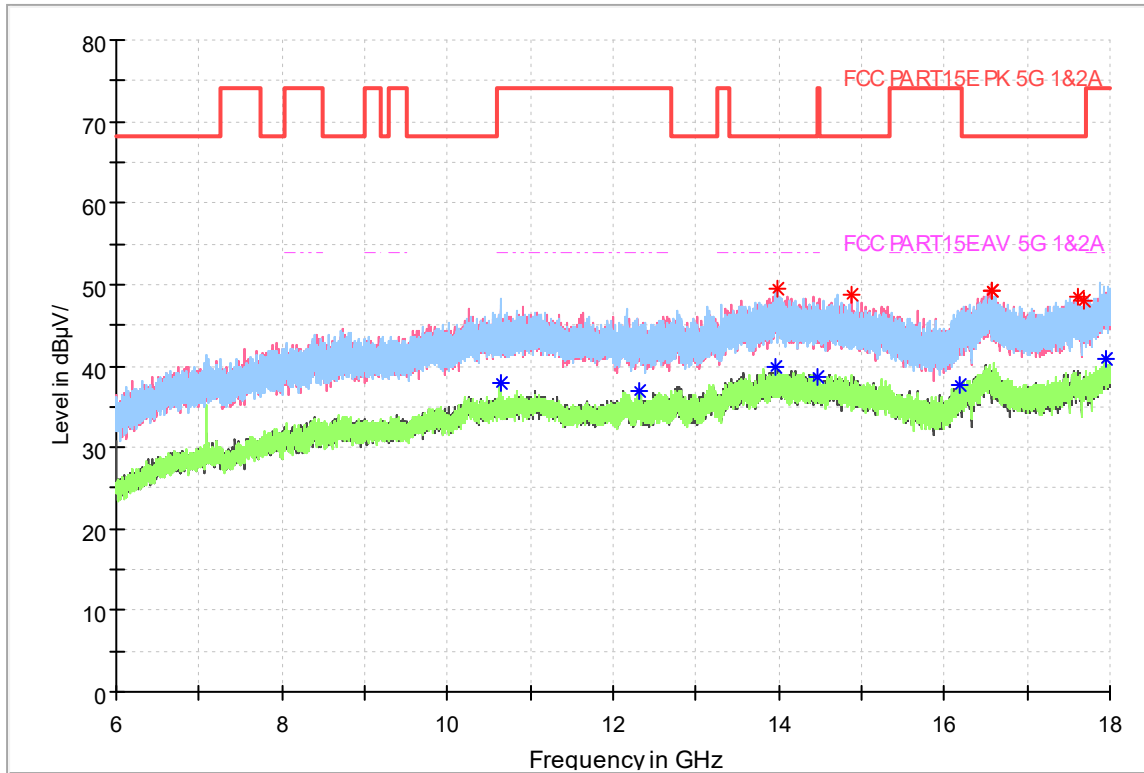
Fig.292 Radiated emission: 802.11n(40M),CH62, 6GHz-18GHz
