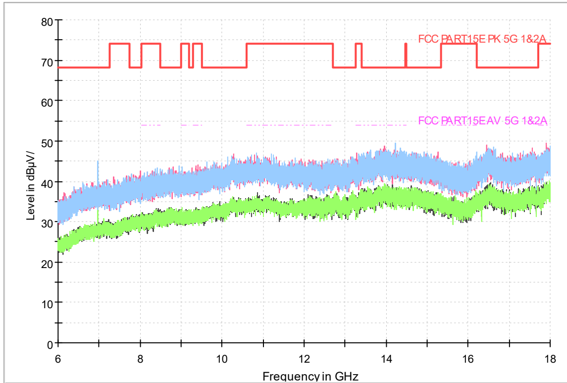
Fig.304 Radiated emission: 802.11ac(20M),CH36, 6GHz-18GHz
