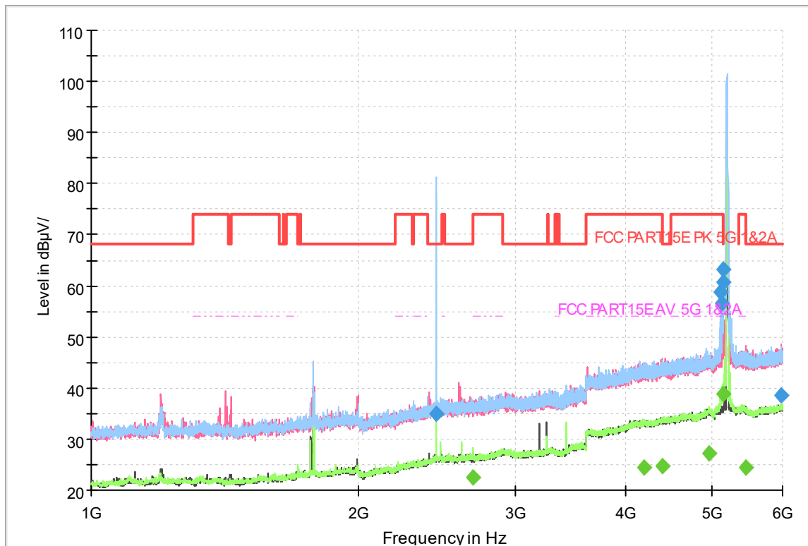
Fig.305 Radiated emission: 802.11ac(20M),CH40, 1GHz-6GHz
