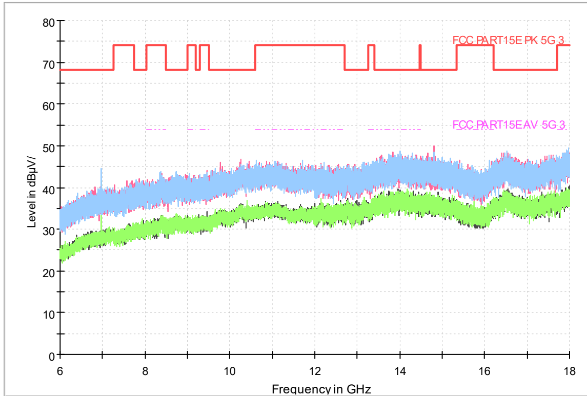
Fig.302 Radiated emission: 802.11n(40M),CH159, 6GHz-18GHz
