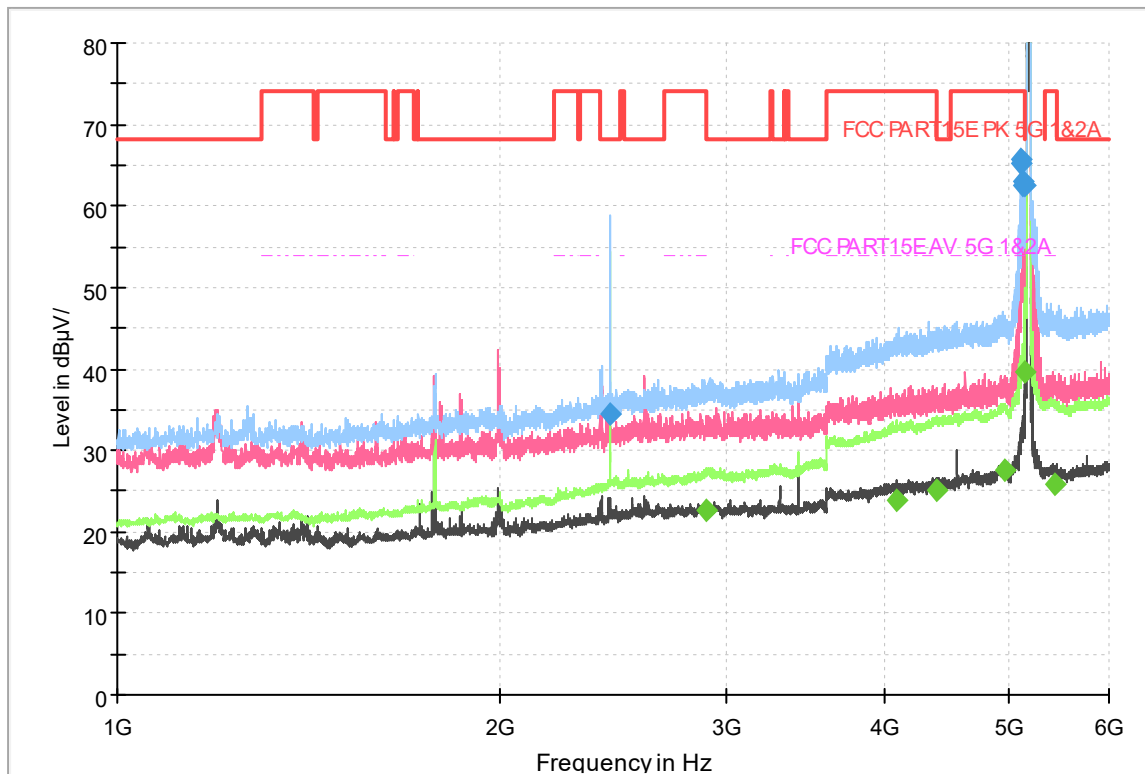
Fig.285 Radiated emission: 802.11n(40M),CH38, 1GHz-6GHz
