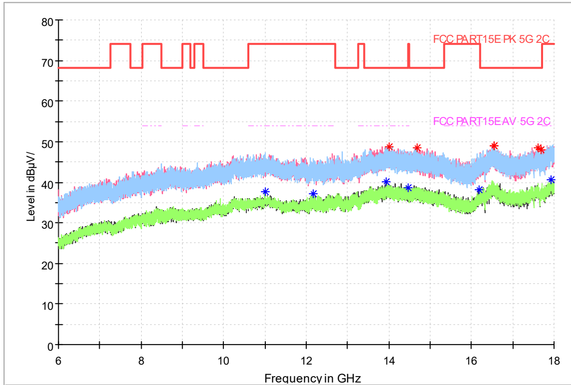
Fig.296 Radiated emission: 802.11n(40M),CH118, 6GHz-18GHz
