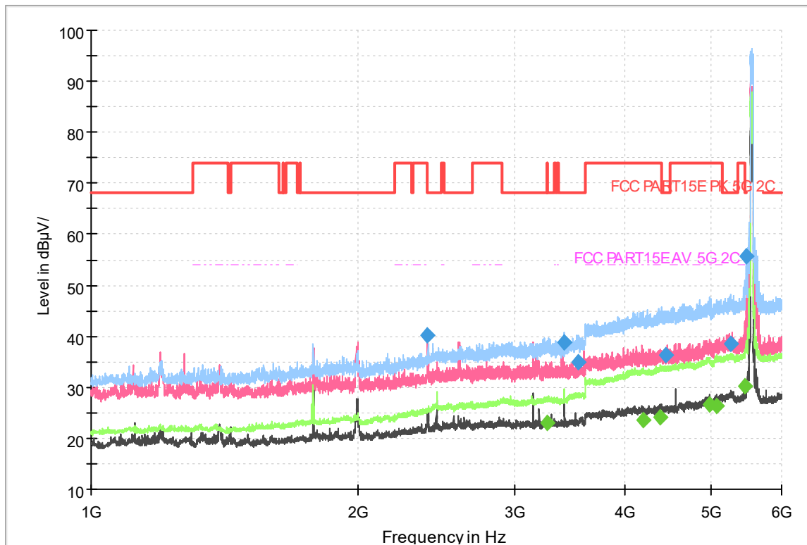
Fig.295 Radiated emission: 802.11n(40M),CH118, 1GHz-6GHz
