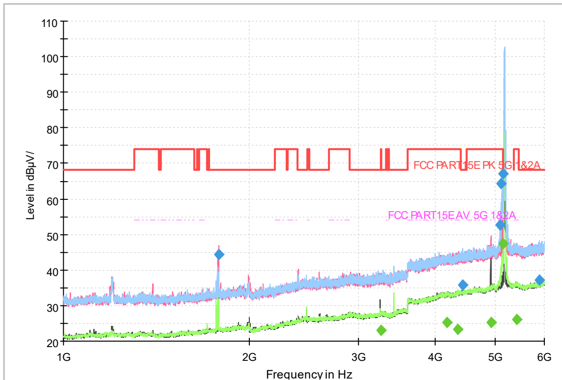
Fig.303 Radiated emission: 802.11ac(20M),CH36, 1GHz-6GHz
