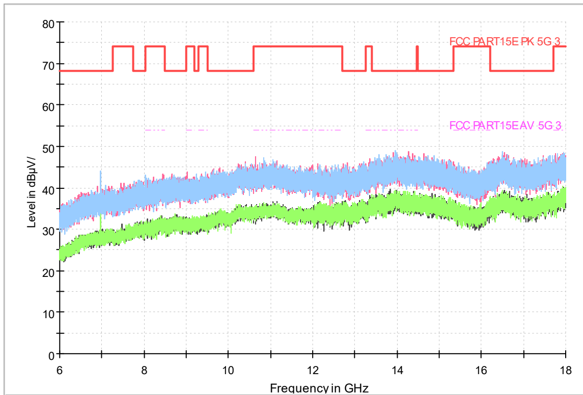
Fig.280 Radiated emission: 802.11n(20M),CH149, 6GHz-18GHz
