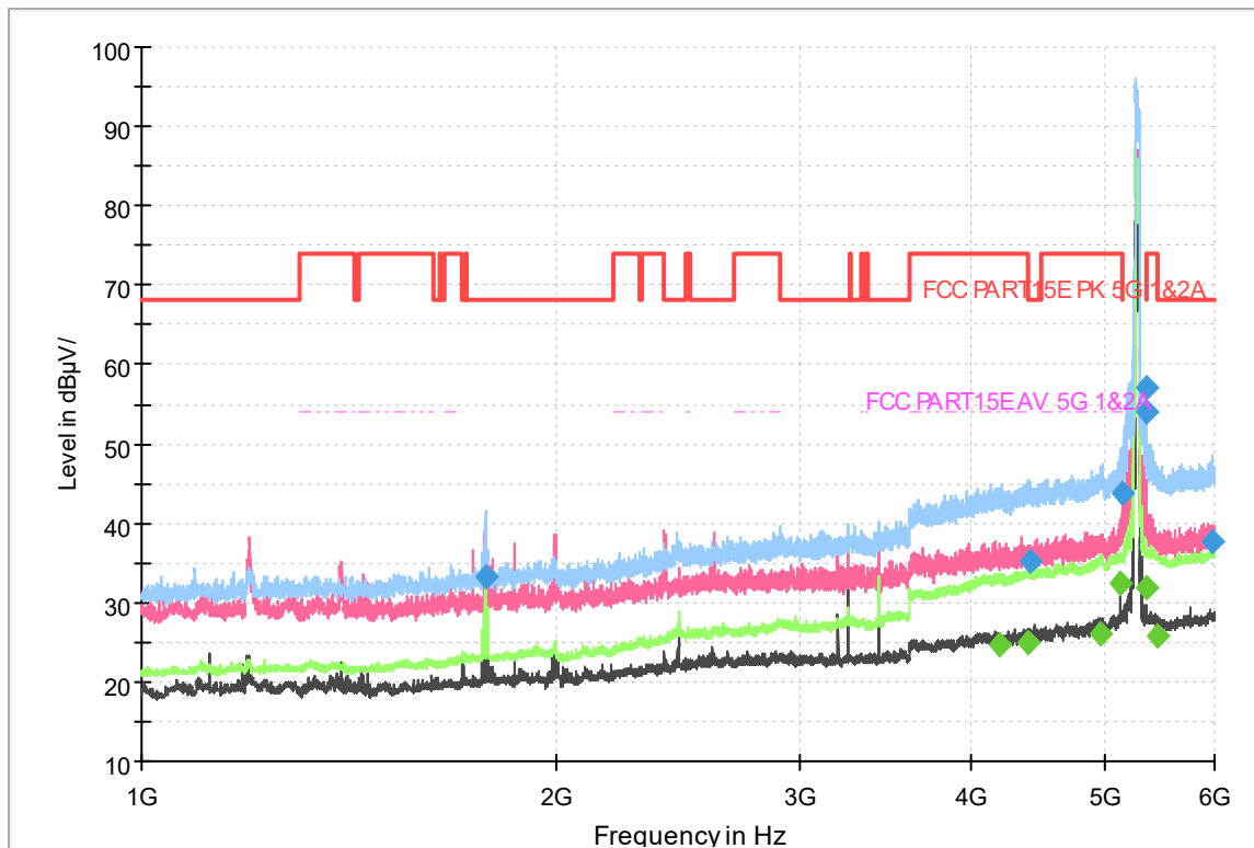
Fig.289 Radiated emission: 802.11n(40M),CH54, 1GHz-6GHz
