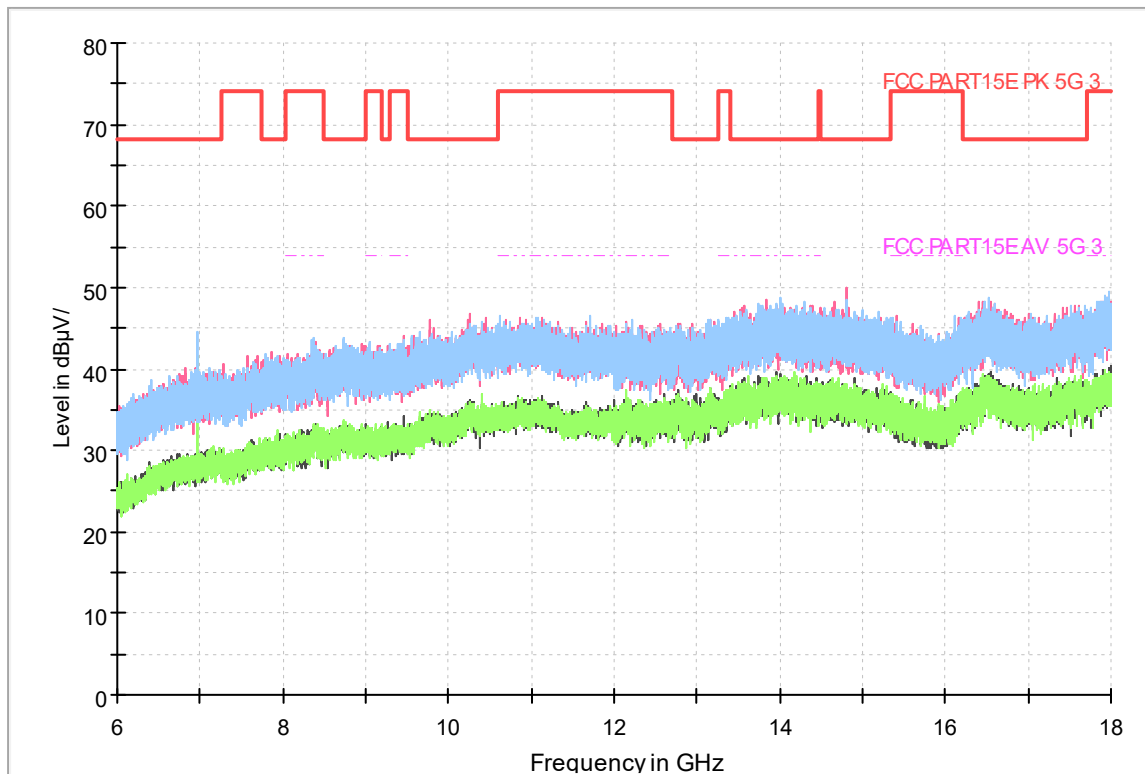
Fig.300 Radiated emission: 802.11n(40M),CH151, 6GHz-18GHz
