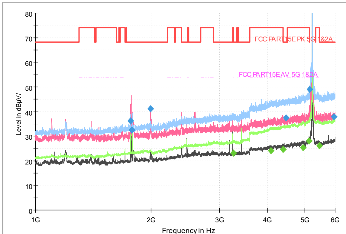
Fig.307 Radiated emission: 802.11ac(20M),CH48, 1GHz-6GHz
