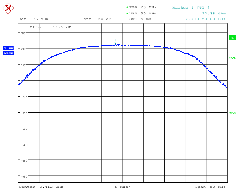
Fig.42 Peak Conducted Output Power CH1, 11n, MCS5
