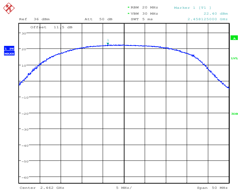
Fig.56 Peak Conducted Output Power CH11, 11n, MCS3
