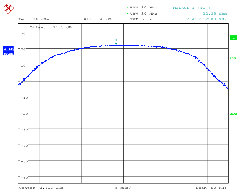
Fig.40 Peak Conducted Output Power CH1, 11n, MCS3
