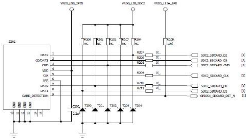
Figure 4.33: SD Card Interface Circuit
