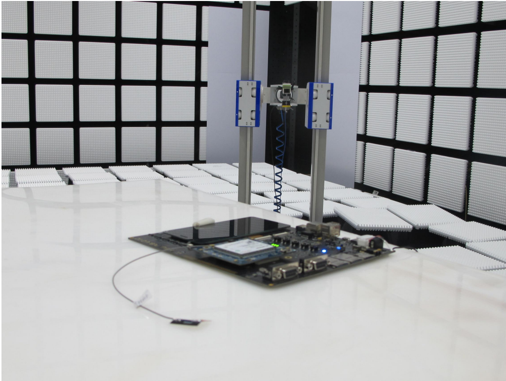
Pic3. Radiated emissions (18GHz-26.5GHz)
