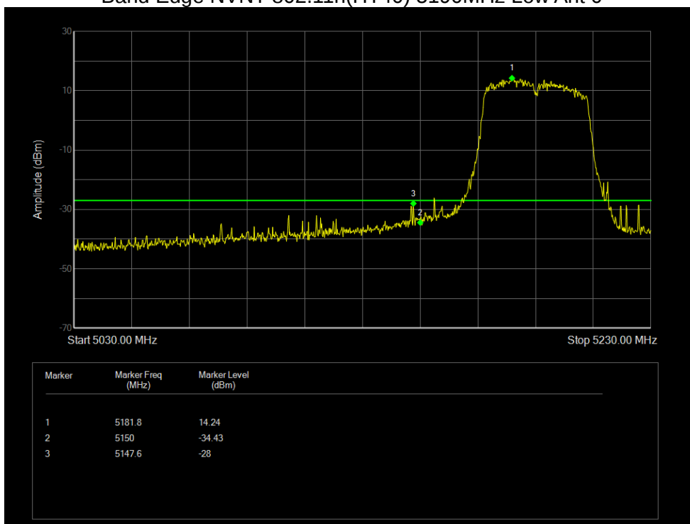
Band Edge NVNT 802.11n(HT40) 5190MHz Low Ant 0
