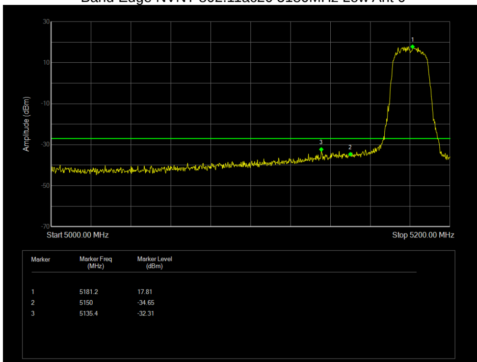
Band Edge NVNT 802.11ac20 5180MHz Low Ant 0
