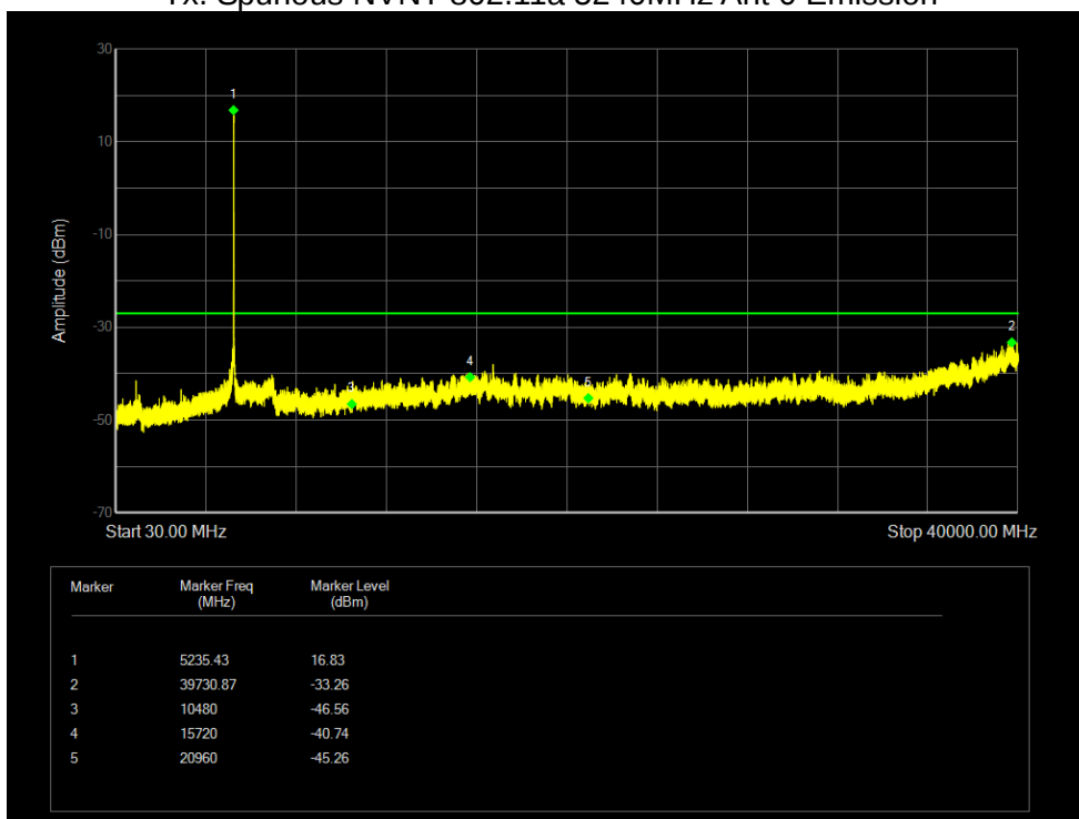
Tx. Spurious NVNT 802.11a 5240MHz Ant 0 Emission
