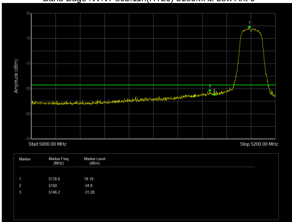
Band Edge NVNT 802.11n(HT20) 5180MHz Low Ant 0
