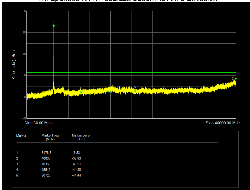
Tx. Spurious NVNT 802.11a 5180MHz Ant 0 Emission
