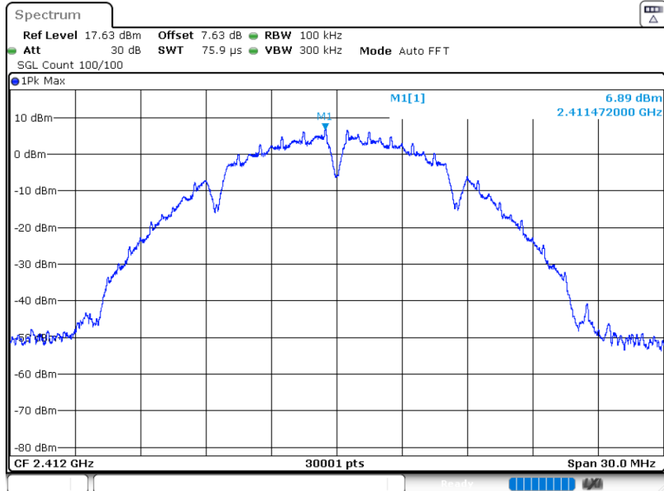
Tx. Spurious NVNT 802.11b 2412MHz Ant 0 Ref
