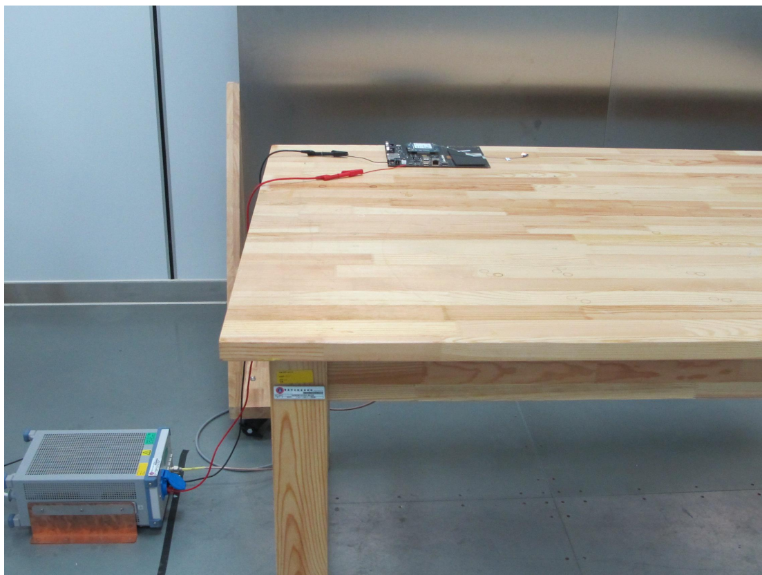
Pic5. Conducted emission
