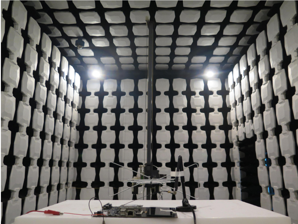
Pic3. Radiated spurious emission (30MHz-1GHz)
