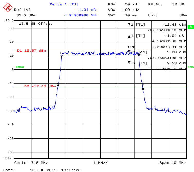
QPSK (5 MHz) - 99% Occupied & 26 dB Emissions Bandwidth, Middle channel
