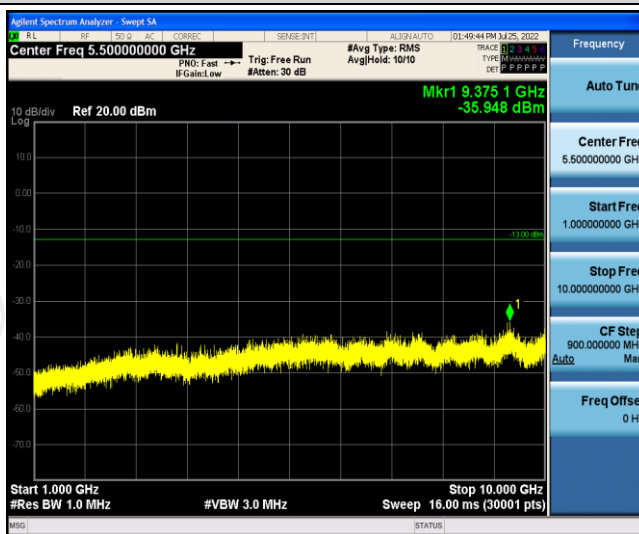
Band26-15MHz-16QAM-26765-1RB#0-Range2:1000~10000MHz
